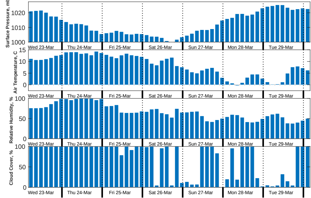
Met Forecast for US Wind VC-207 from 23-Mar-2022 06:00:00 to 30-Mar-2022 06:00:00
