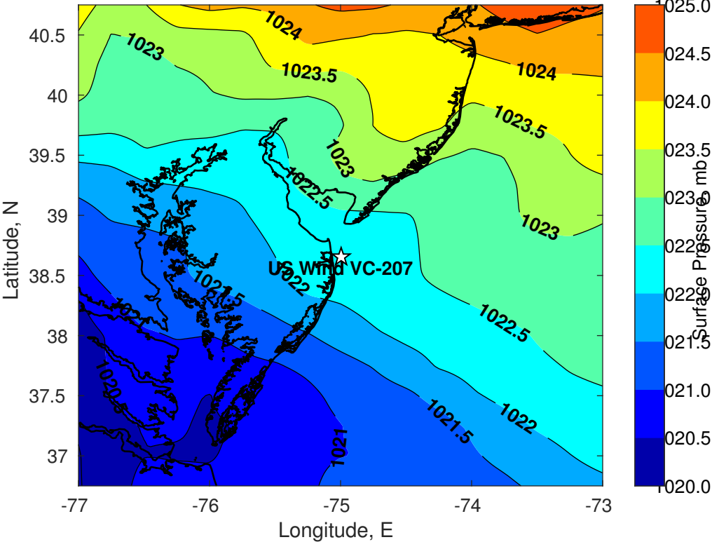
Surface Pressure (mb) for US Wind VC-207 at 23-Mar-2022 06:00:00
