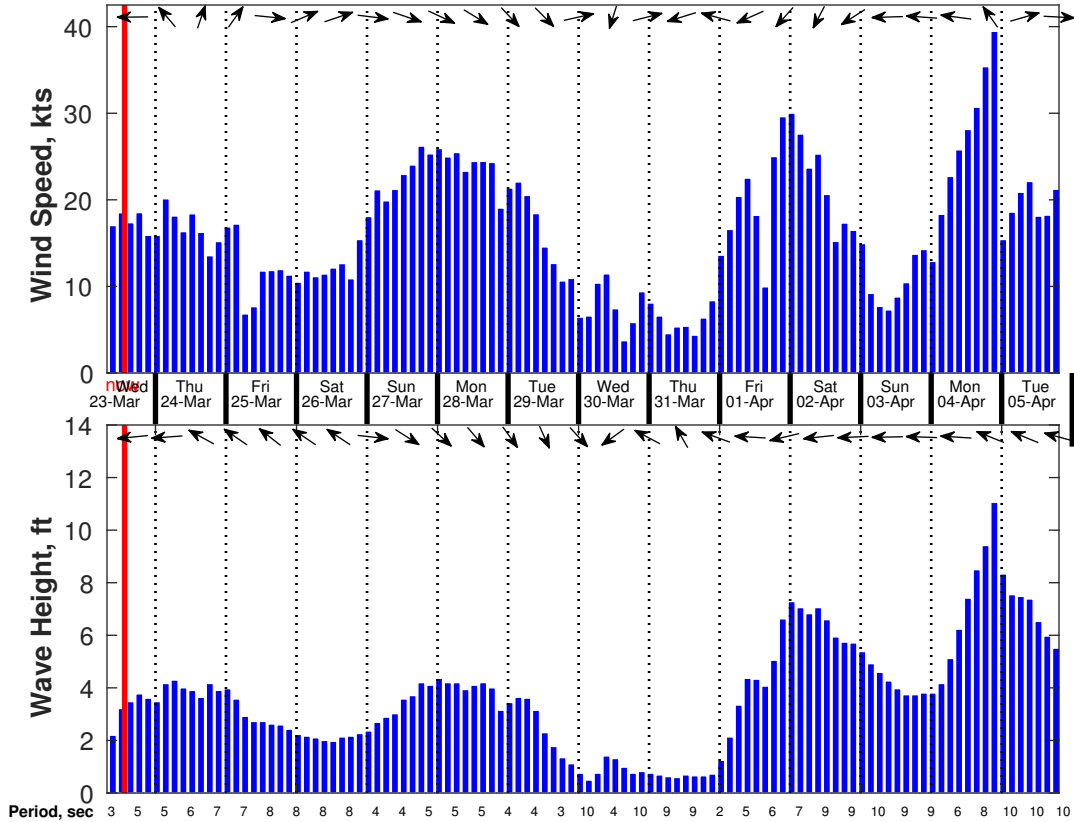
Wind & Wave Forecast for US Wind VC-207 from 23-Mar-2022 08:00:00 to 06-Apr-2022 02:00:00
