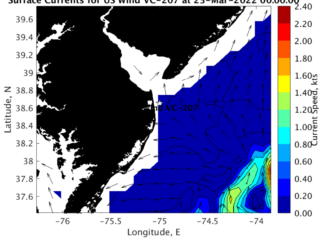
Surface Currents for US Wind VC-207 at 23-Mar-2022 00:00:00
