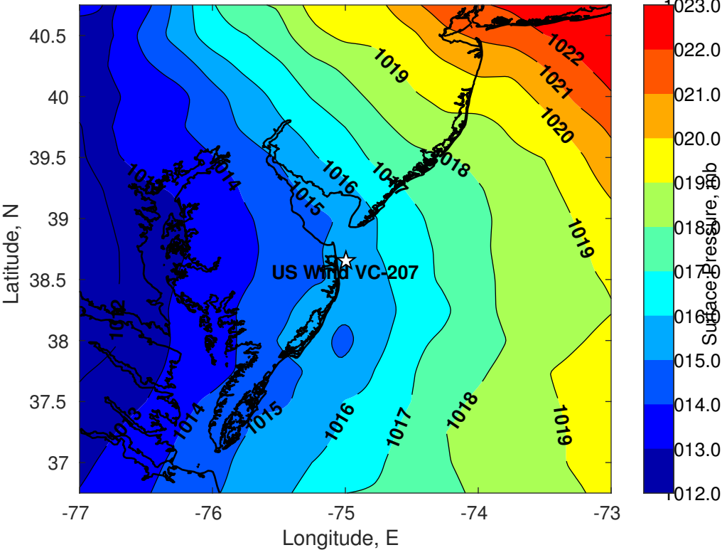
Surface Pressure (mb) for US Wind VC-207 at 24-Mar-2022 03:00:00
