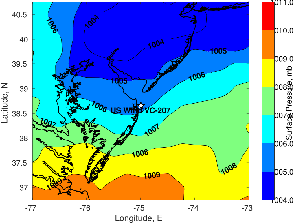
Surface Pressure (mb) for US Wind VC-207 at 25-Mar-2022 03:00:00
