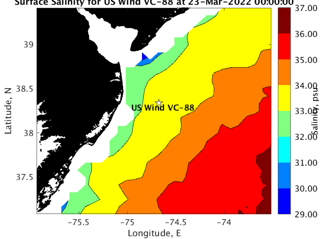
Surface Salinity for US Wind VC-88 at 23-Mar-2022 00:00:00
