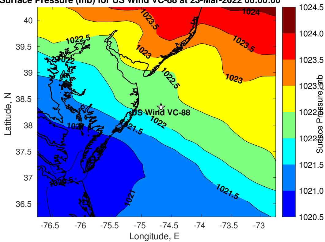
Surface Pressure (mb) for US Wind VC-88 at 23-Mar-2022 06:00:00
