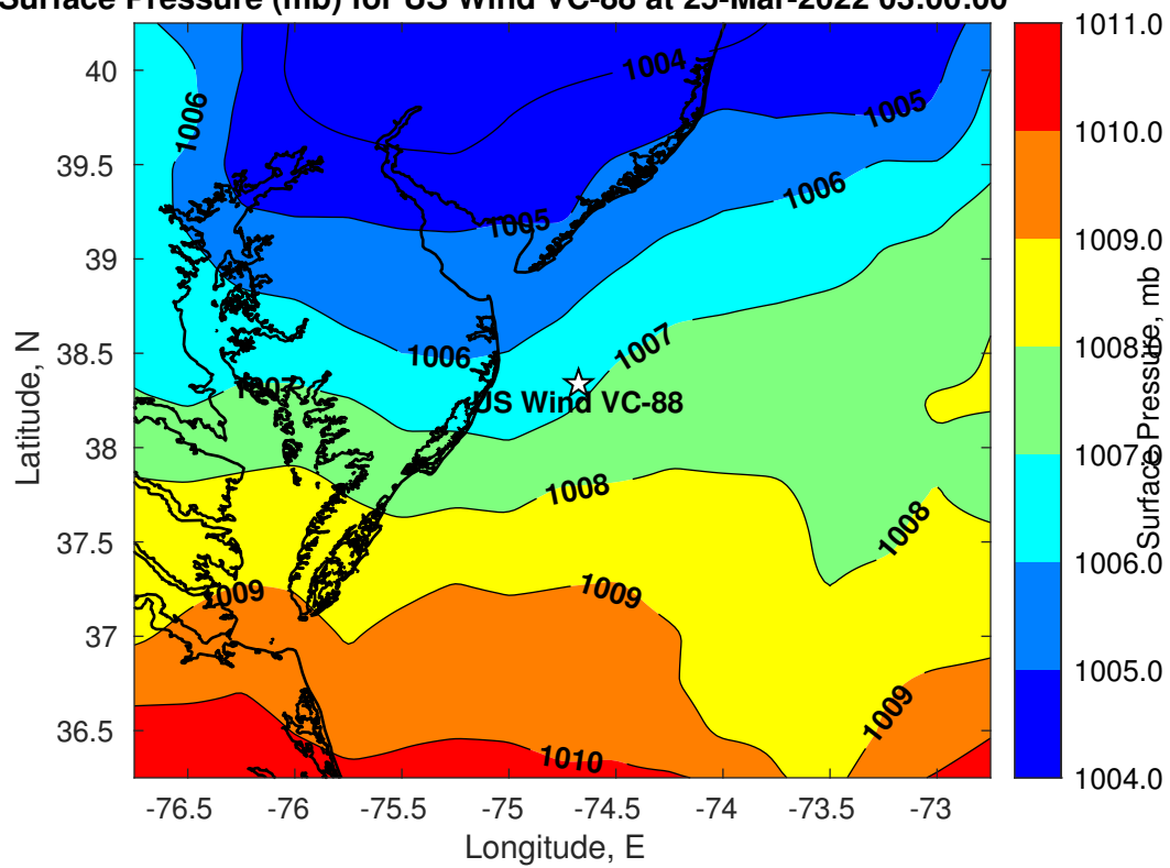
Surface Pressure (mb) for US Wind VC-88 at 25-Mar-2022 03:00:00
