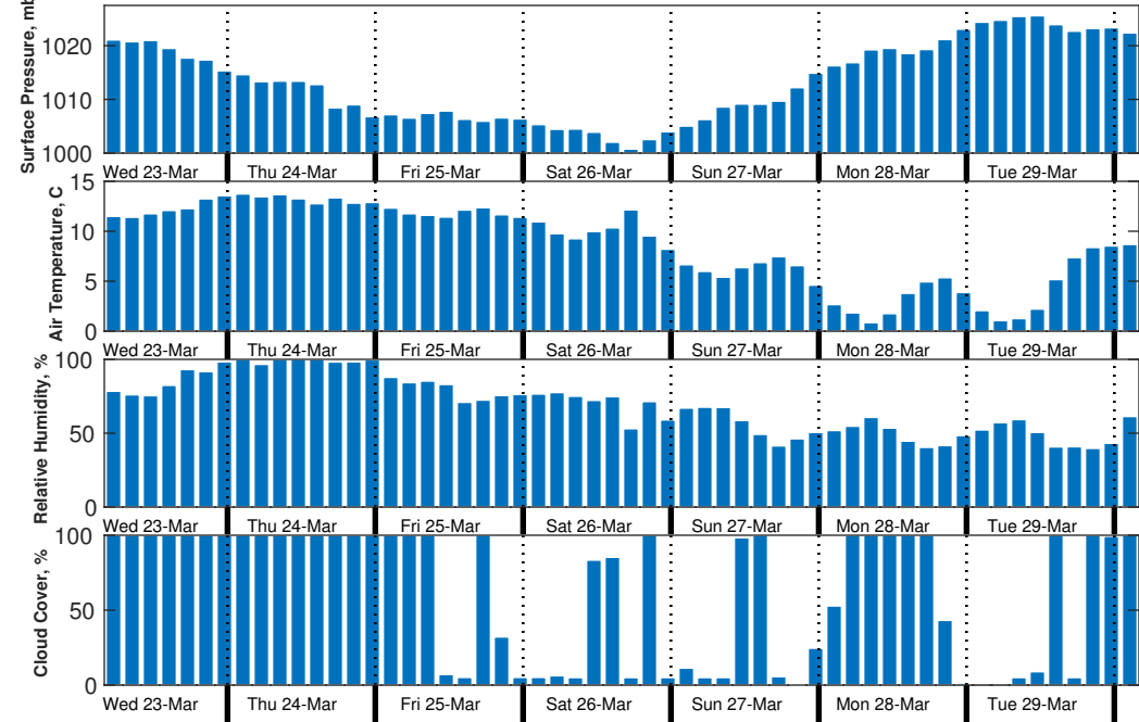
Met Forecast for US Wind VC-88 from 23-Mar-2022 06:00:00 to 30-Mar-2022 06:00:00
