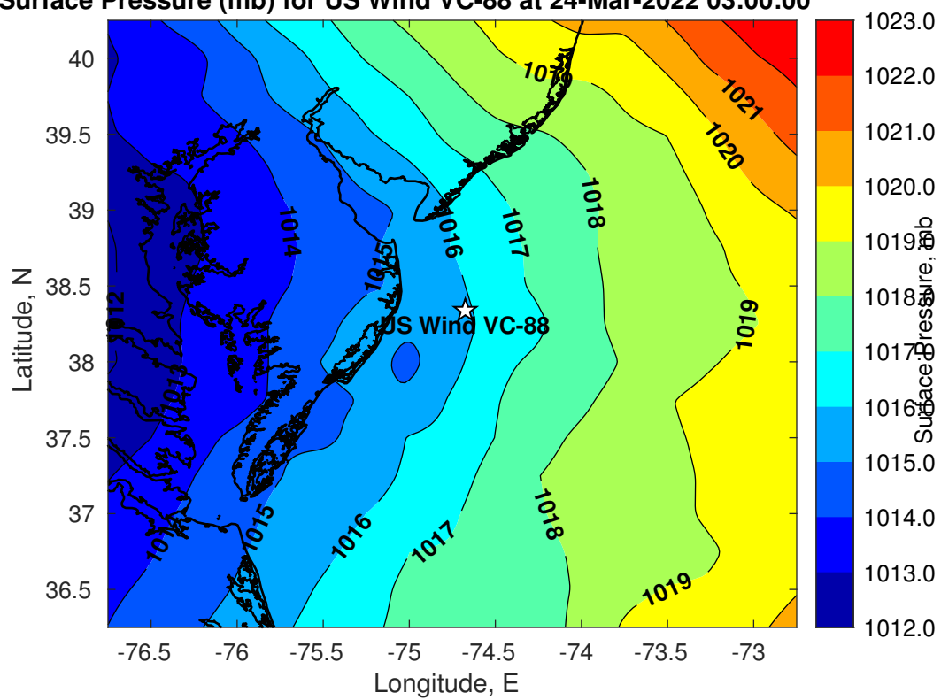
Surface Pressure (mb) for US Wind VC-88 at 24-Mar-2022 03:00:00
