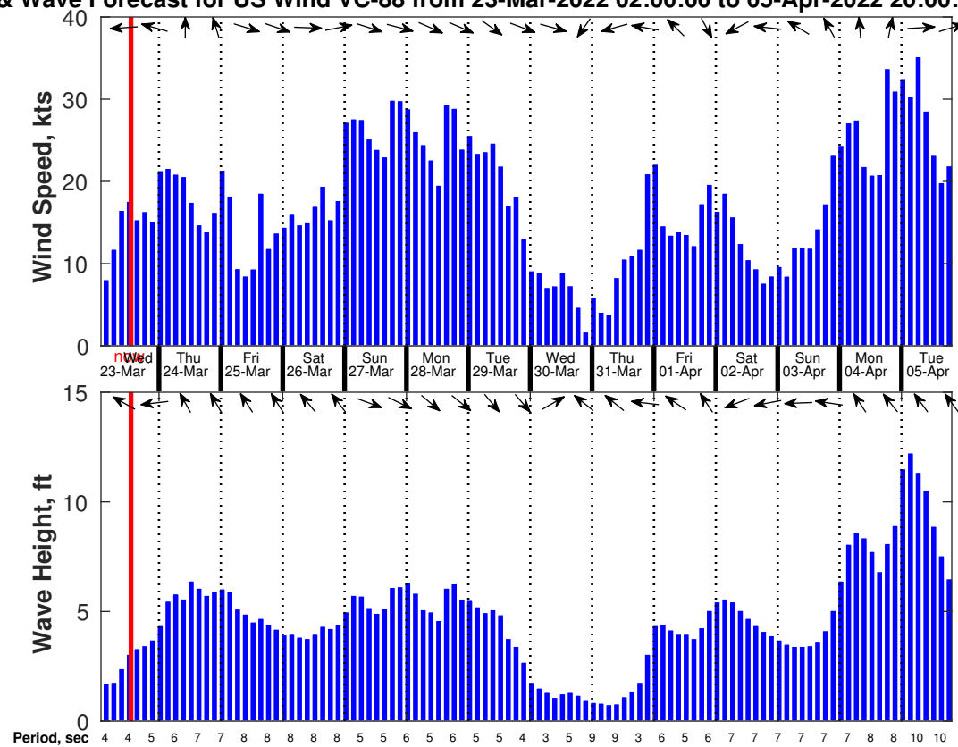
Wind & Wave Forecast for US Wind VC-88 from 23-Mar-2022 02:00:00 to 05-Apr-2022 20:00:00
