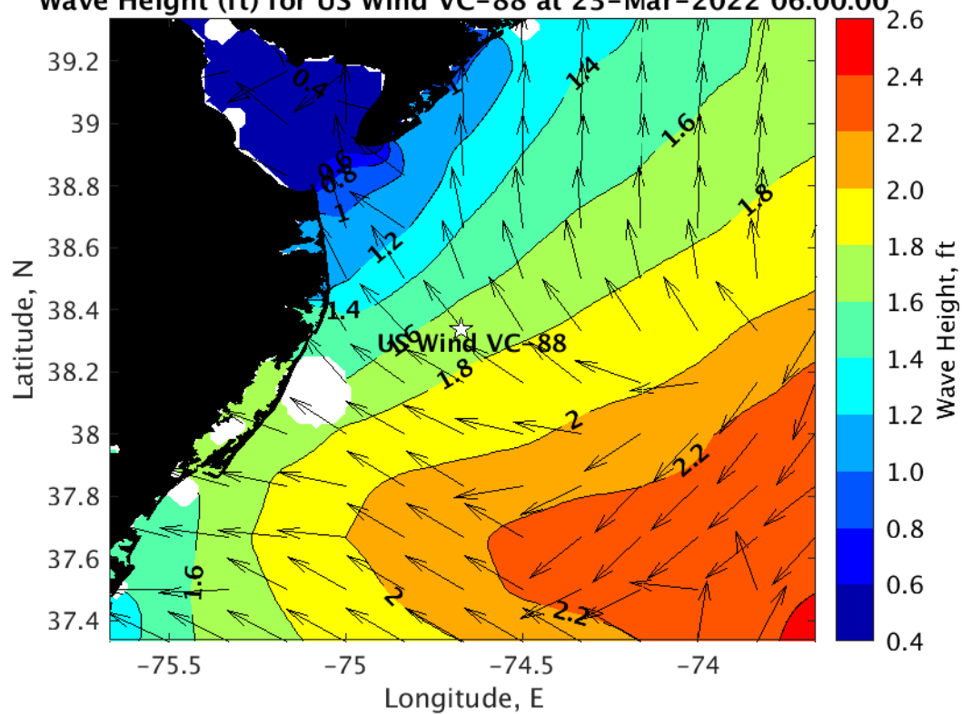
Wave Height (ft) for US Wind VC-88 at 23-Mar-2022 06:00:00
