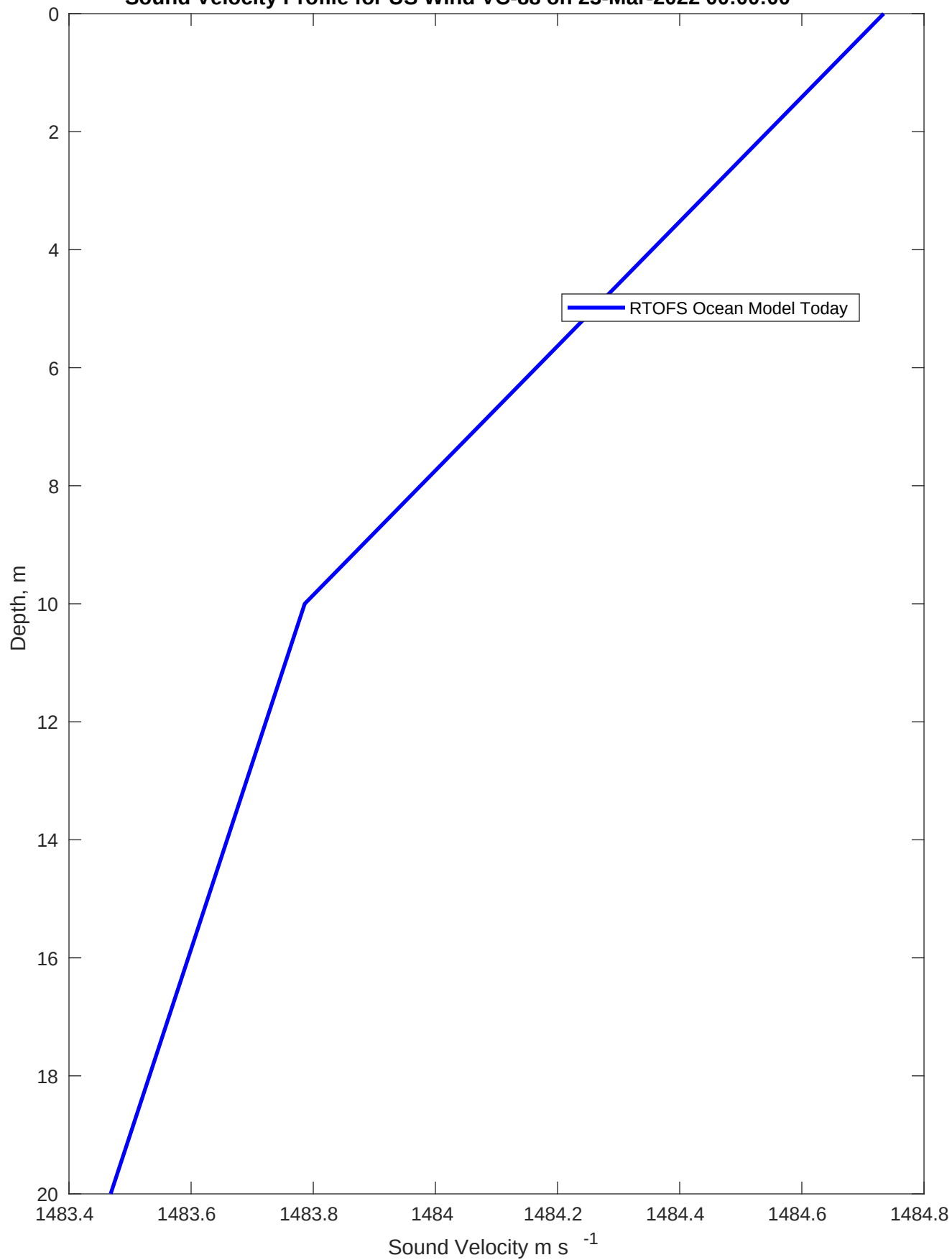
Sound Velocity Profile for US Wind VC-88 on 23-Mar-2022 00:00:00
