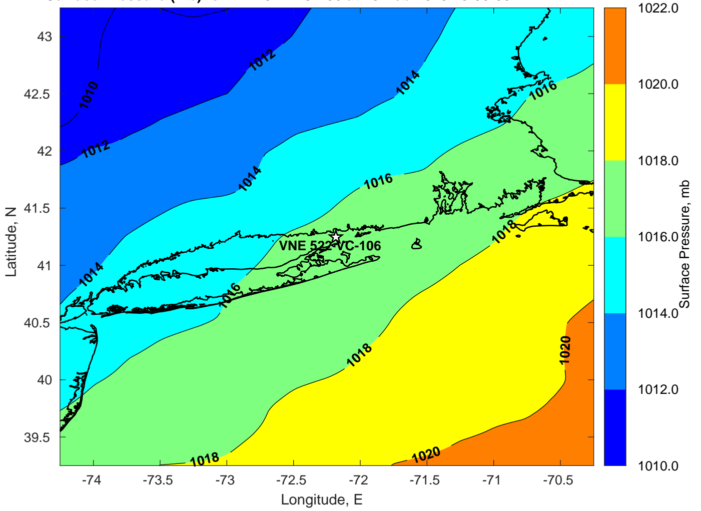
Surface Pressure (mb) for VNE 522 VC-106 at 15-Feb-2023 18:00:00
