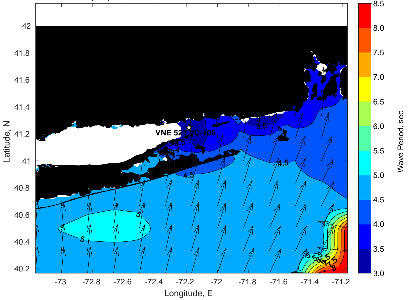
Wave Period (sec) for VNE 522 VC-106 at 15-Feb-2023 18:00:00
