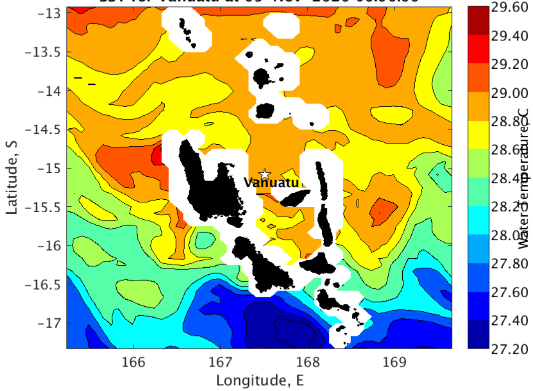
SST for Vanuatu at 05-Nov-2020 00:00:00
