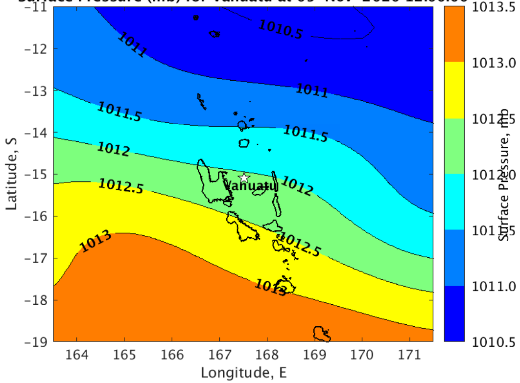
Surface Pressure (mb) for Vanuatu at 05-Nov-2020 12:00:00
