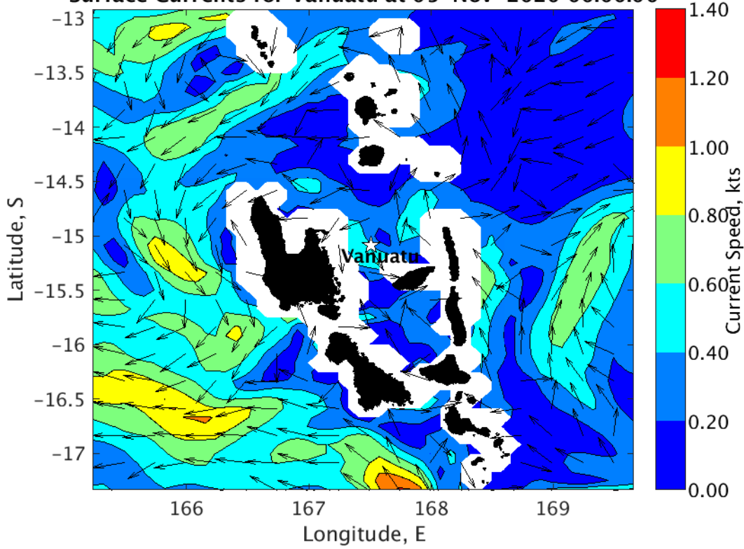
Surface Currents for Vanuatu at 05-Nov-2020 00:00:00
