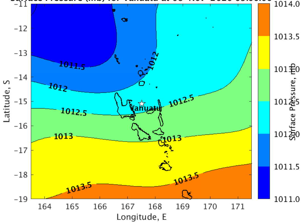
Surface Pressure (mb) for Vanuatu at 06-Nov-2020 09:00:00
