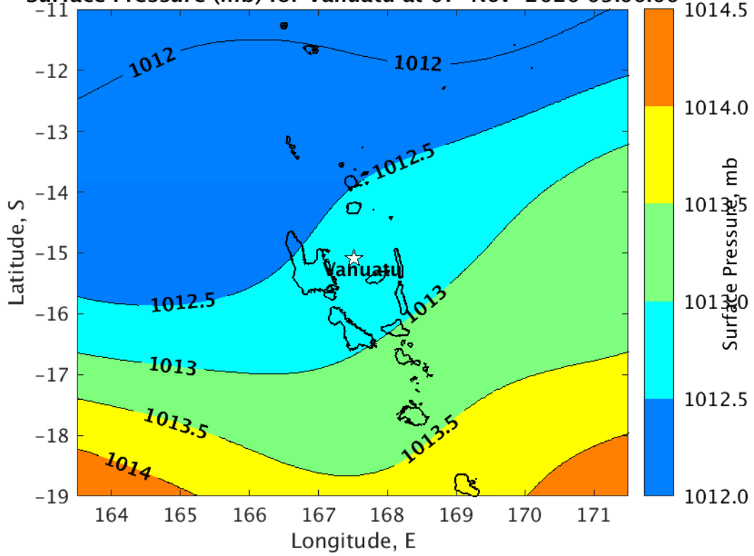
Surface Pressure (mb) for Vanuatu at 07-Nov-2020 09:00:00
