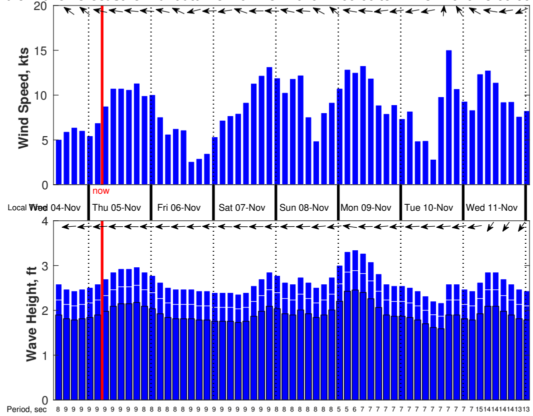
Wind & Wave Forecast for Vanuatu from 04-Nov-2020 11:00:00 to 11-Nov-2020 23:00:00
