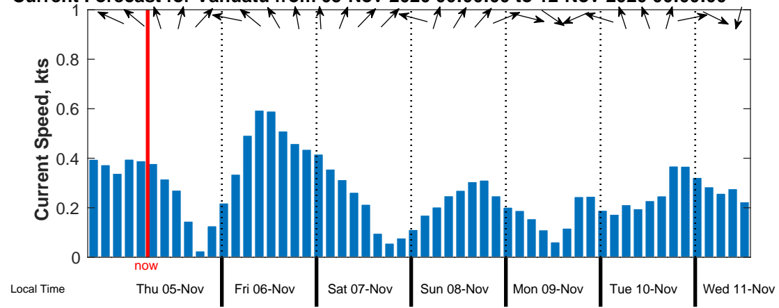
Current Forecast for Vanuatu from 05-Nov-2020 00:00:00 to 12-Nov-2020 00:00:00
