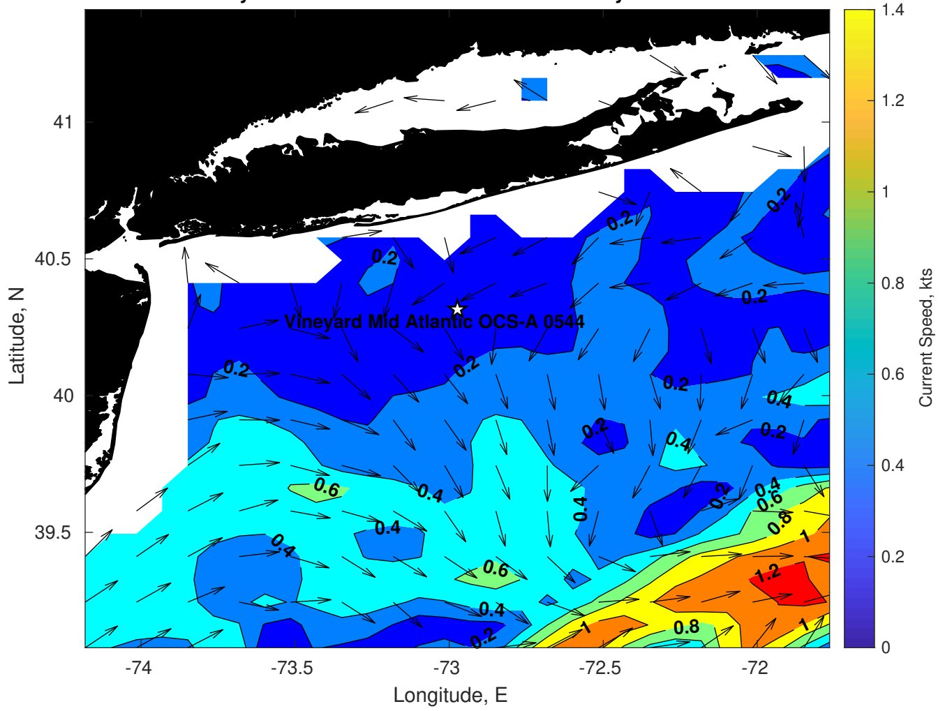
Surface Currents for Vineyard Mid Atlantic OCS-A 0544 at 03-May-2024 00:00:00
