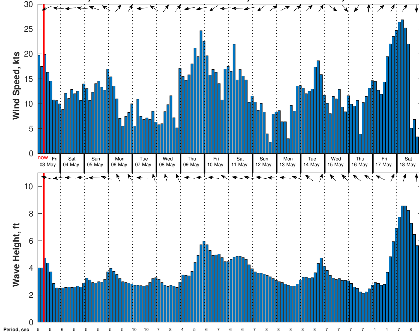
Wind & Wave Forecast for Vineyard Mid Atlantic OCS-A 0544 from 03-May-2024 01:00:00 to 19-May-2024 01:00:00
