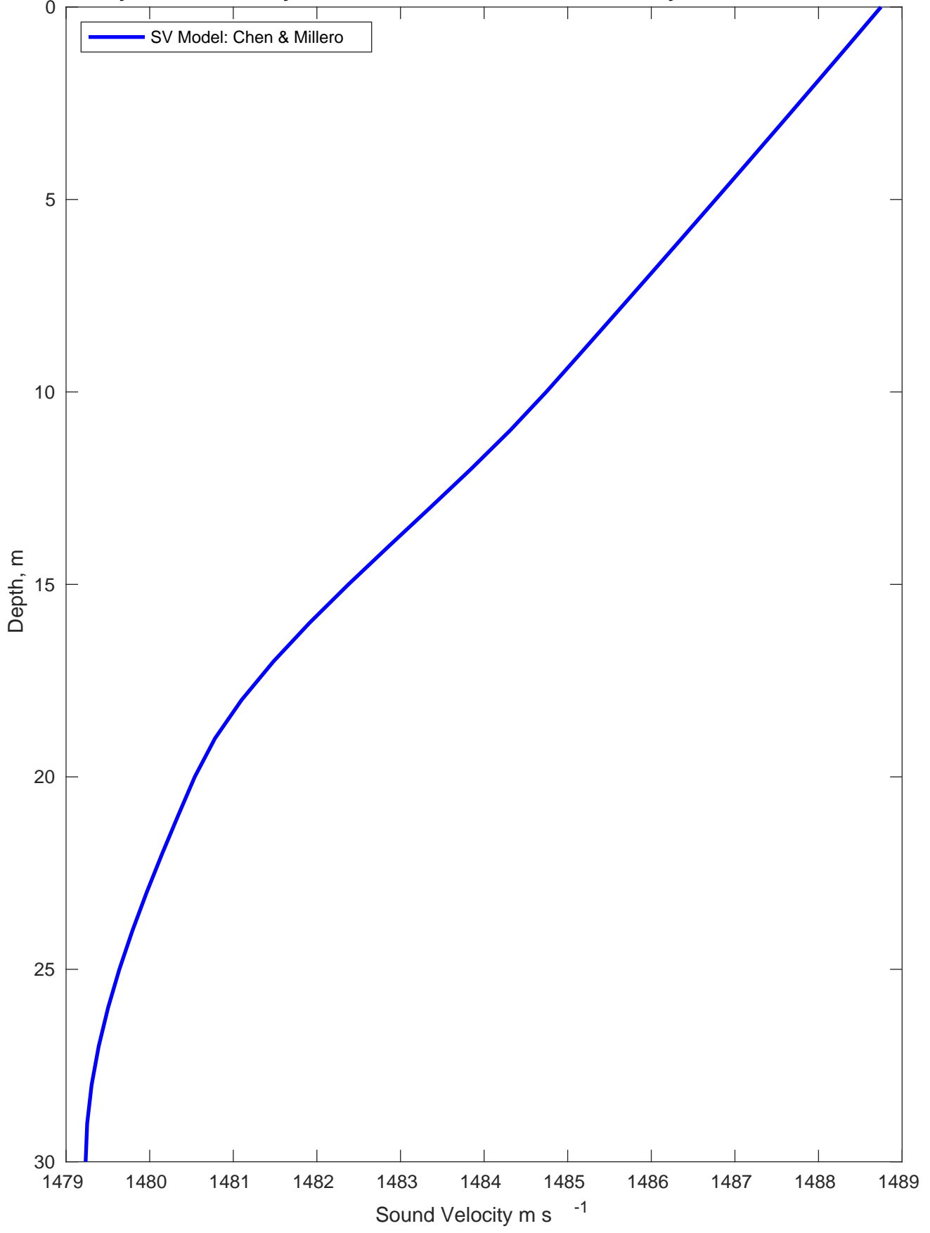
Sound Velocity Profile for Vineyard Mid Atlantic OCS-A 0544 on 03-May-2024 00:00:00
