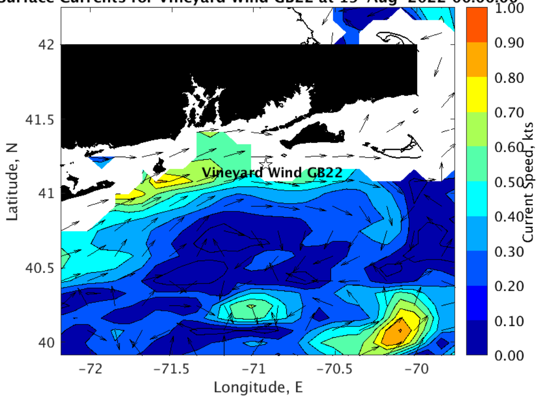
Surface Currents for Vineyard Wind GB22 at 19-Aug-2022 00:00:00
