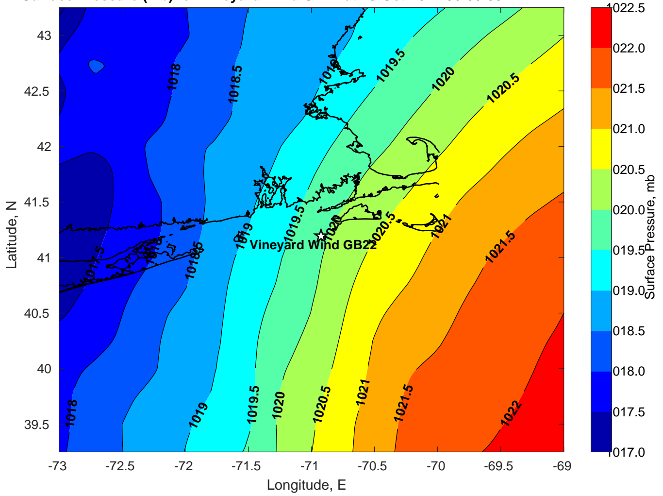
Surface Pressure (mb) for Vineyard Wind GB22 at 13-Oct-2022 06:00:00
