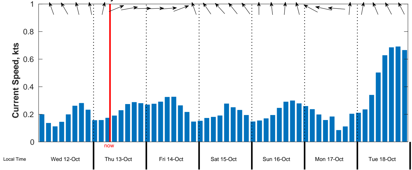
Current Forecast for Vineyard Wind GB22 from 12-Oct-2022 00:00:00 to 19-Oct-2022 00:00:00
