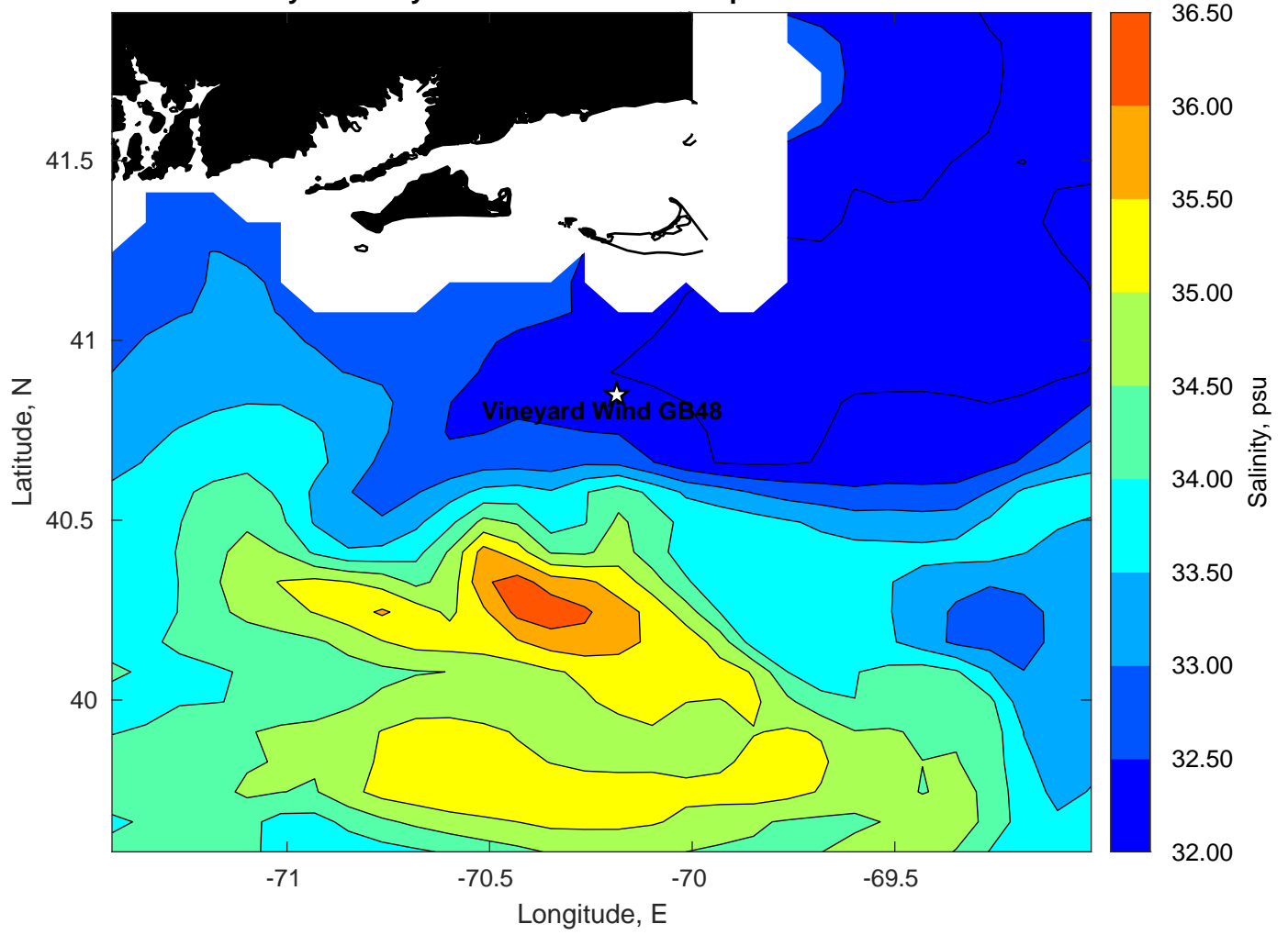
Surface Salinity for Vineyard Wind GB48 at 07-Sep-2022 00:00:00
