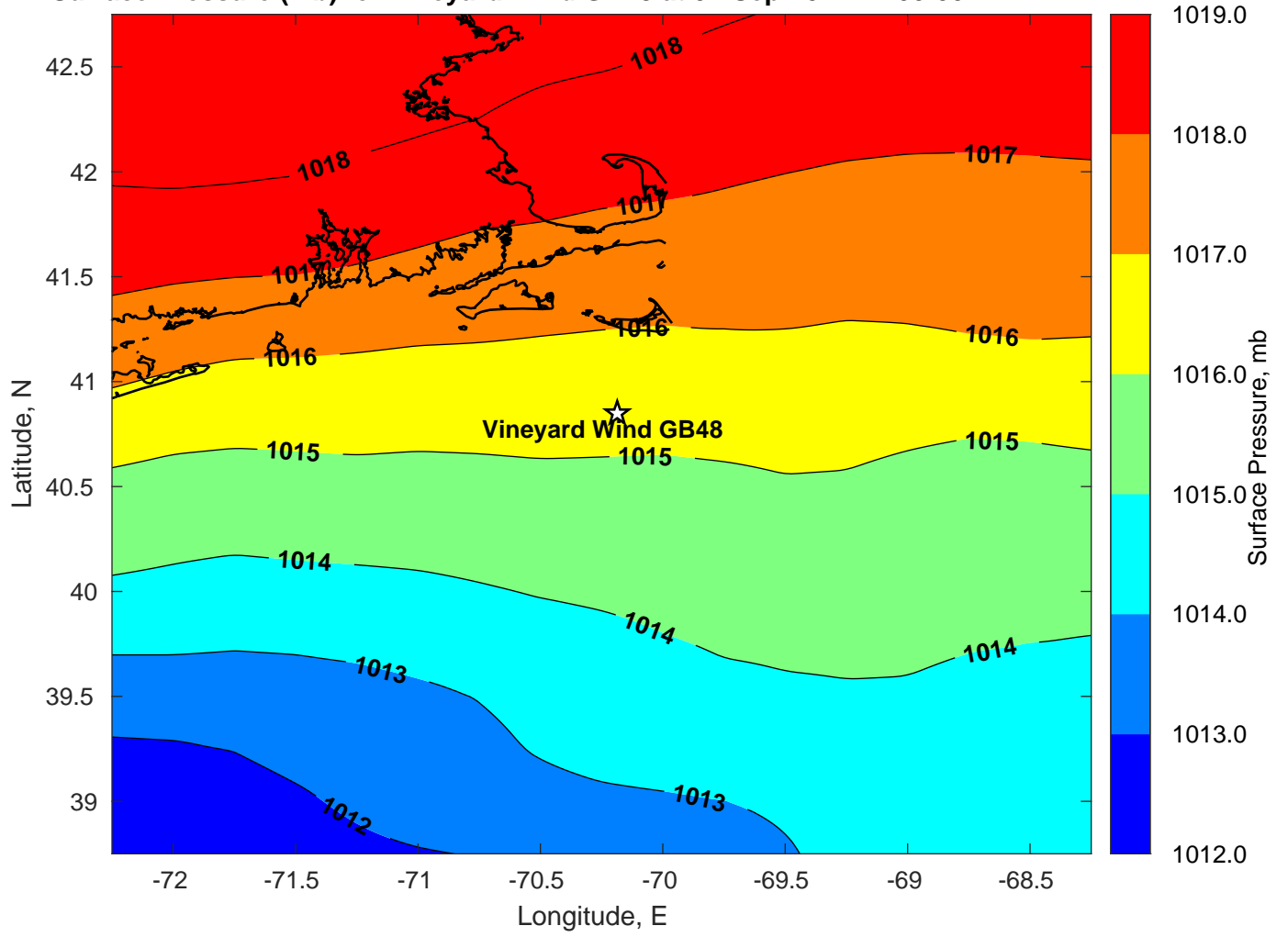
Surface Pressure (mb) for Vineyard Wind GB48 at 07-Sep-2022 12:00:00
