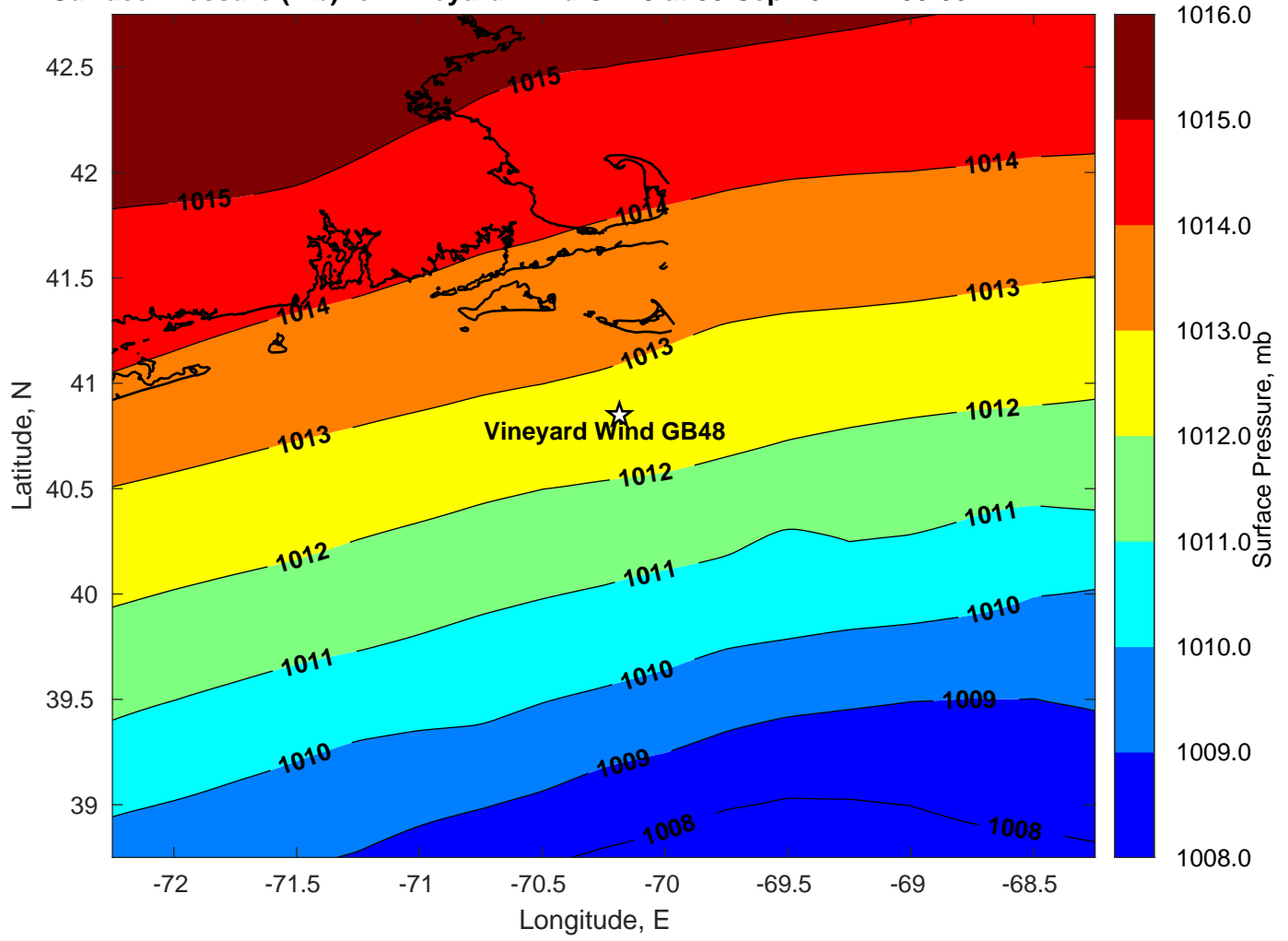
Surface Pressure (mb) for Vineyard Wind GB48 at 08-Sep-2022 12:00:00
