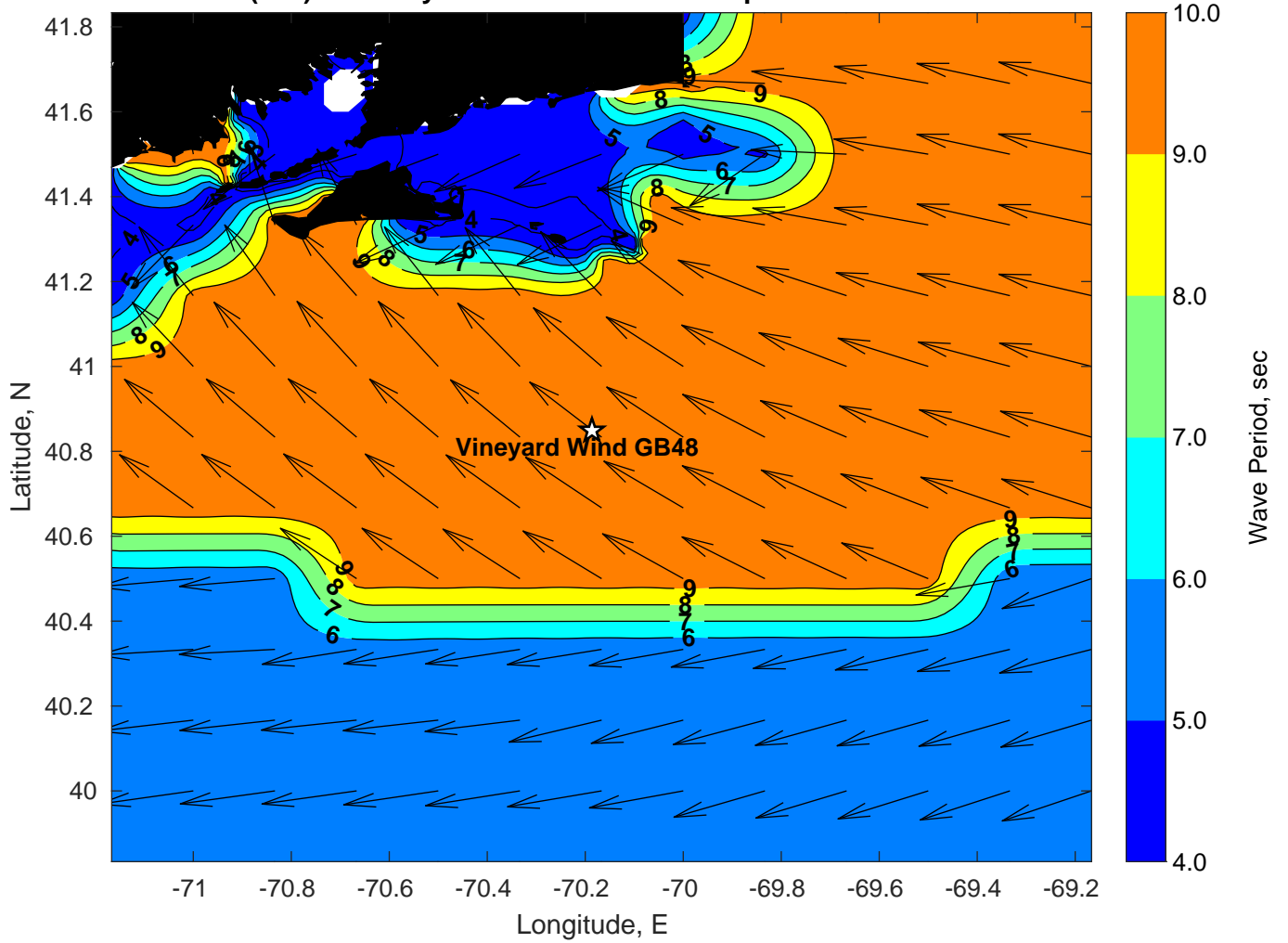
Wave Period (sec) for Vineyard Wind GB48 at 07-Sep-2022 12:00:00
