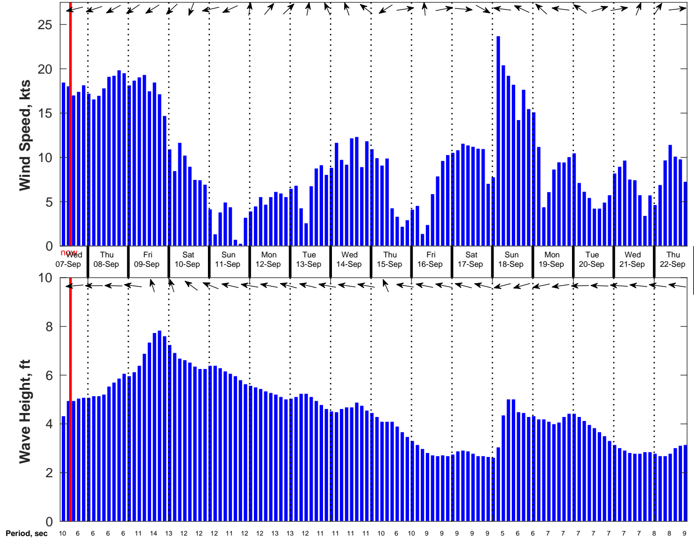
Wind & Wave Forecast for Vineyard Wind GB48 from 07-Sep-2022 08:00:00 to 23-Sep-2022 08:00:00
