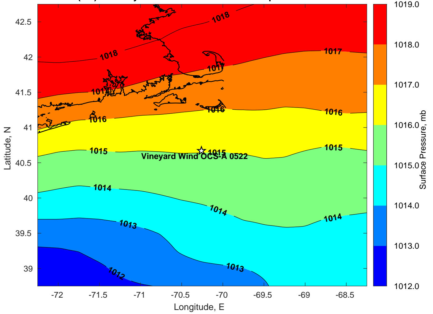
Surface Pressure (mb) for Vineyard Wind OCS-A 0522 at 07-Sep-2022 12:00:00
