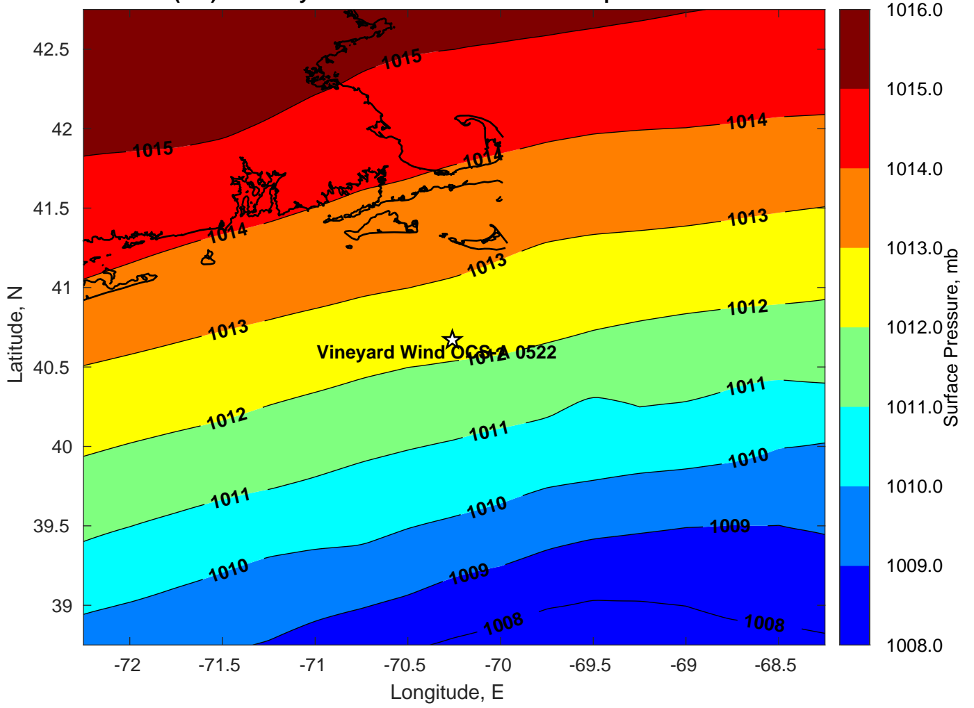
Surface Pressure (mb) for Vineyard Wind OCS-A 0522 at 08-Sep-2022 12:00:00
