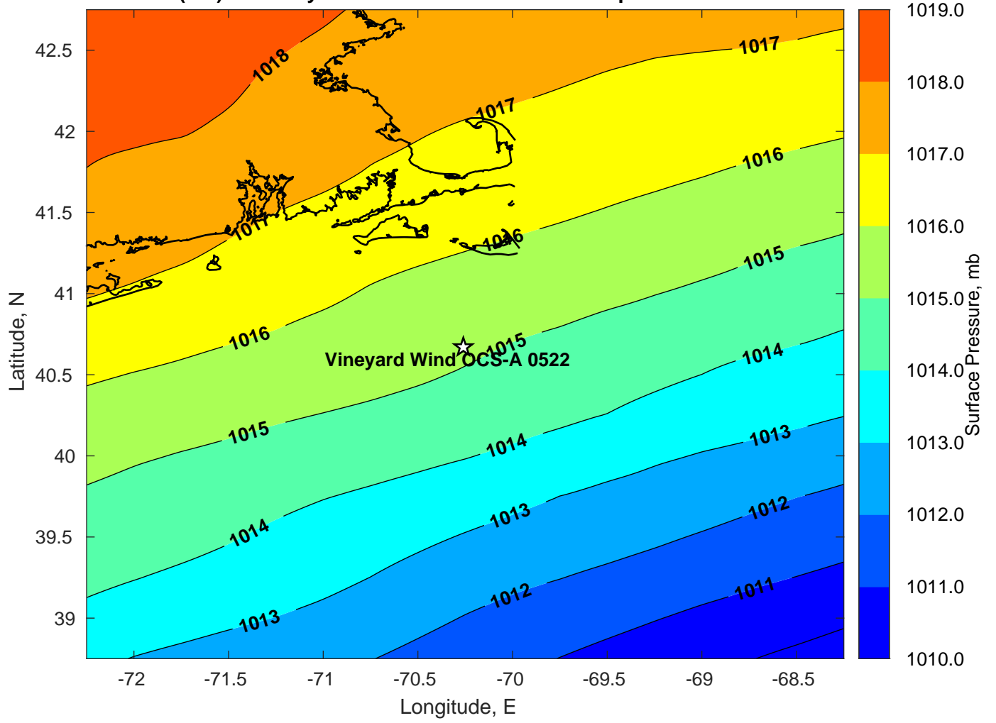
Surface Pressure (mb) for Vineyard Wind OCS-A 0522 at 09-Sep-2022 12:00:00
