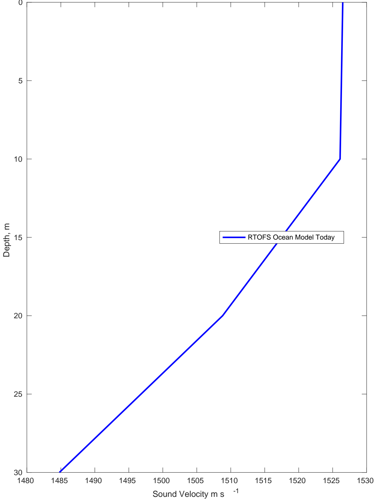
Sound Velocity Profile for Vineyard Wind OCS-A 0522 on 07-Sep-2022 00:00:00
