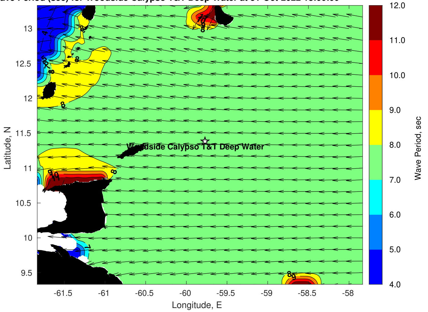
Wave Period (sec) for Woodside Calypso T&T Deep Water at 31-Oct-2022 18:00:00
