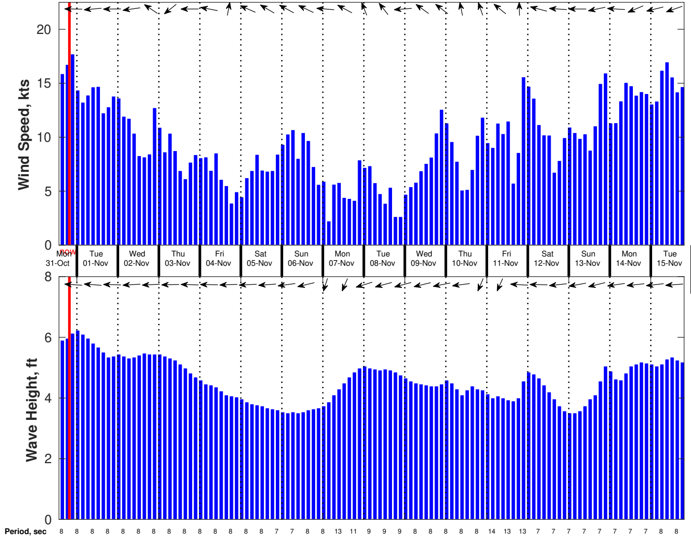
Wind & Wave Forecast for Woodside Calypso T&T Deep Water from 31-Oct-2022 14:00:00 to 16-Nov-2022 14:00:00
