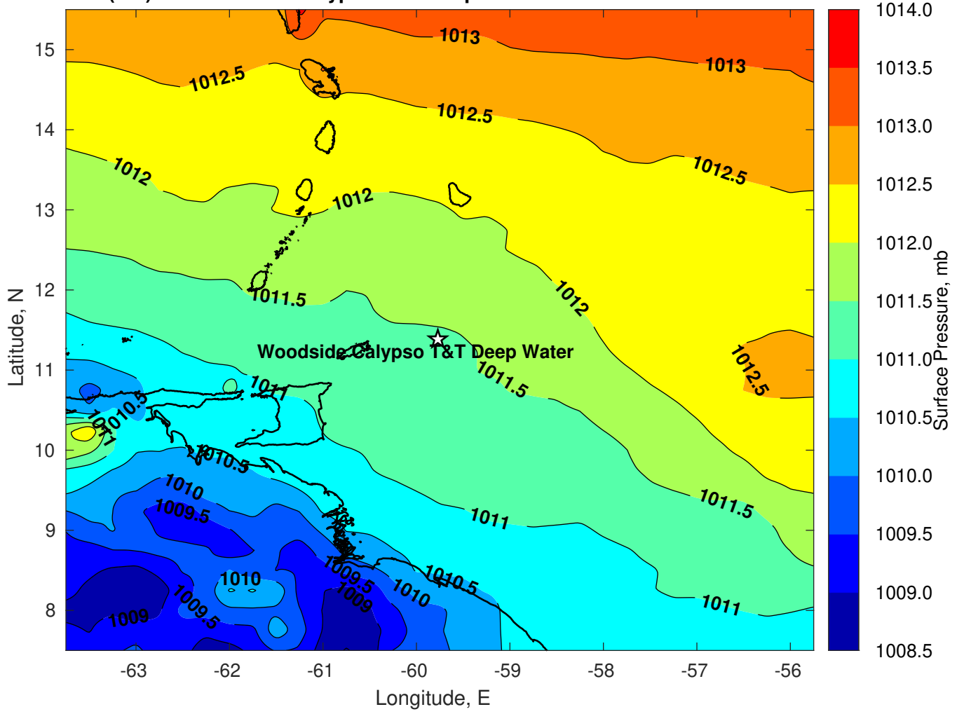
Surface Pressure (mb) for Woodside Calypso T&T Deep Water at 02-Nov-2022 18:00:00
