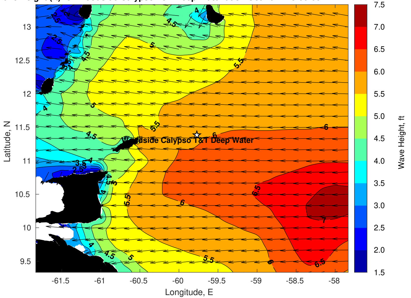
Wave Height (ft) for Woodside Calypso T&T Deep Water at 31-Oct-2022 18:00:00
