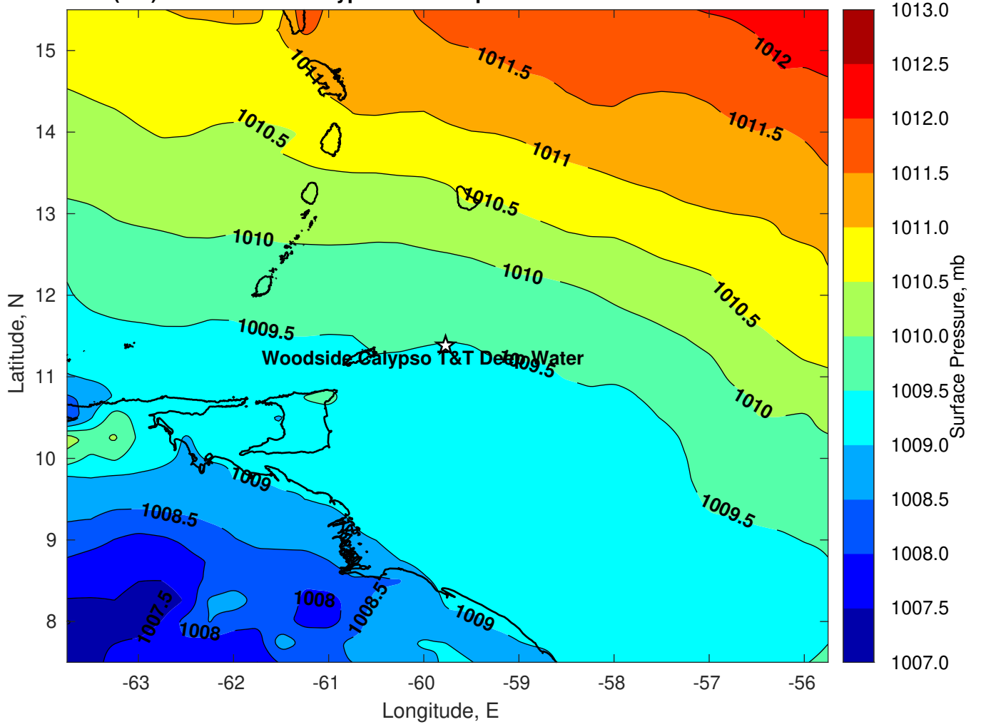
Surface Pressure (mb) for Woodside Calypso T&T Deep Water at 31-Oct-2022 18:00:00
