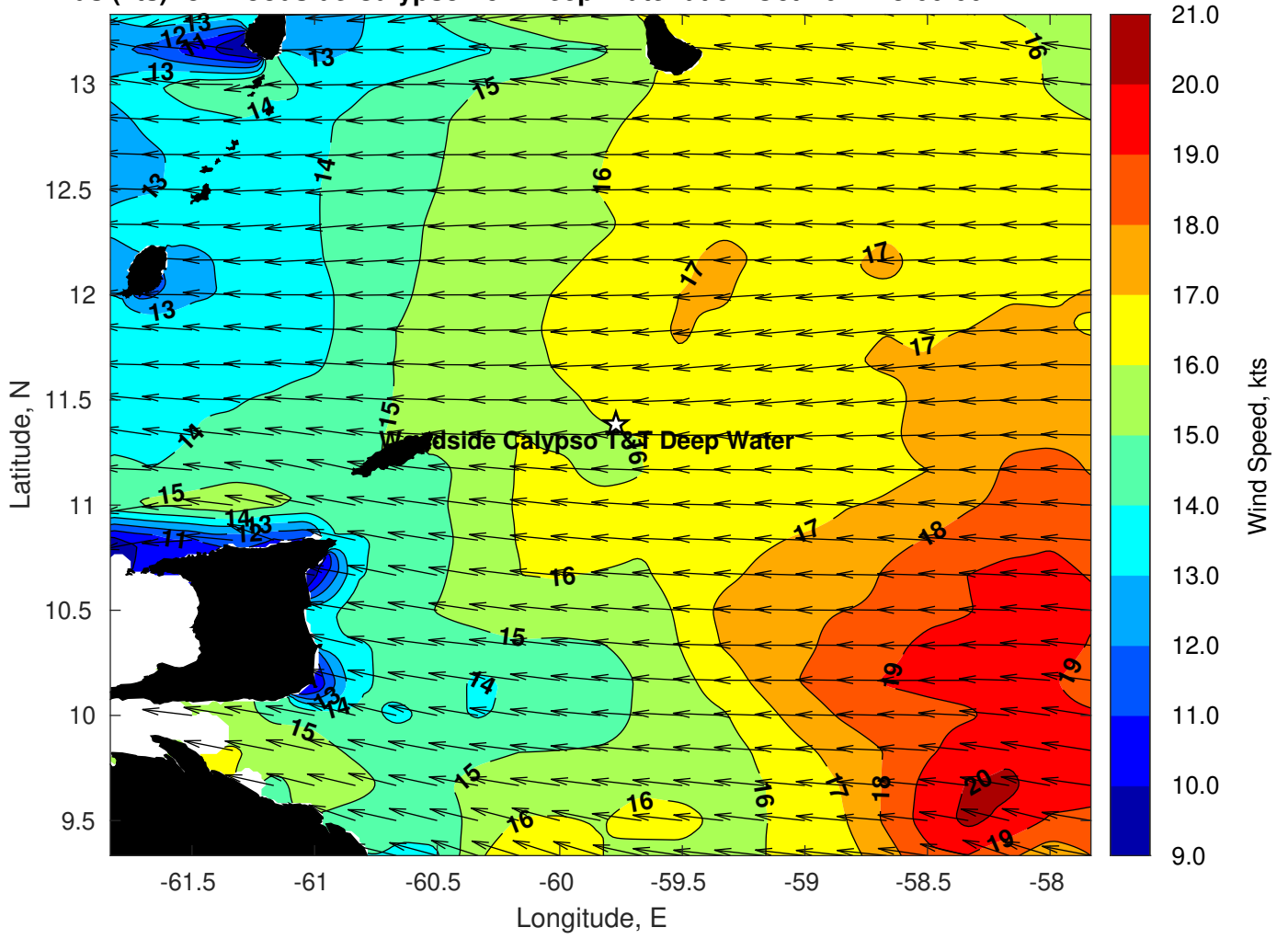
Winds (kts) for Woodside Calypso T&T Deep Water at 31-Oct-2022 18:00:00
