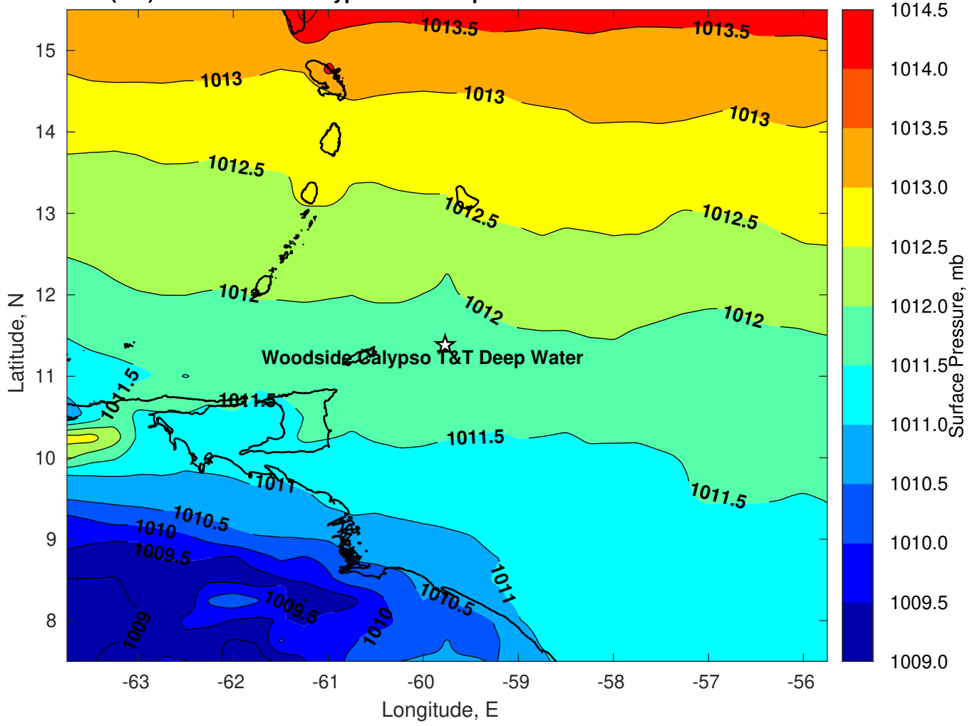
Surface Pressure (mb) for Woodside Calypso T&T Deep Water at 01-Nov-2022 18:00:00
