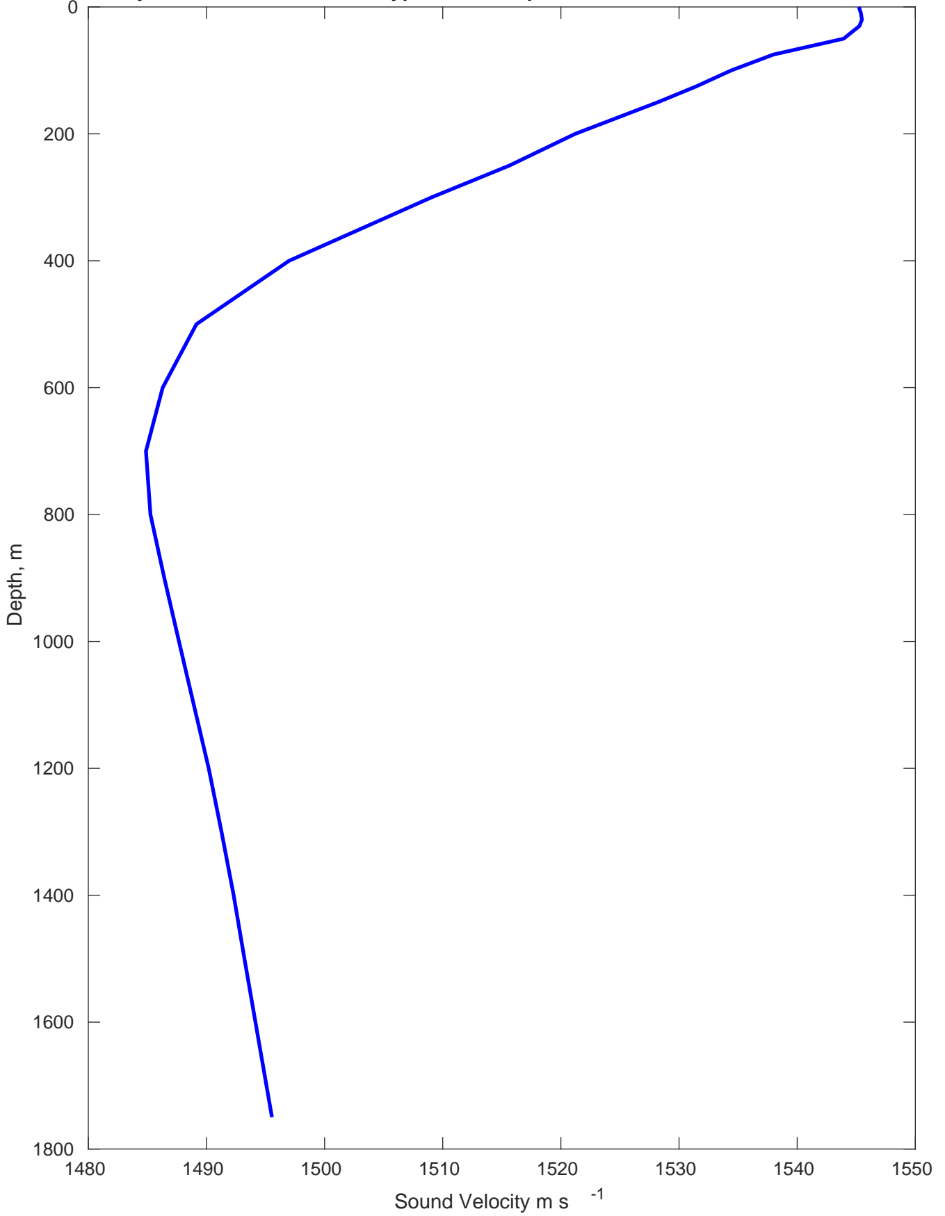
Sound Velocity Profile for Woodside Calypso T&T Deep Water on 31-Oct-2023 00:00:00
