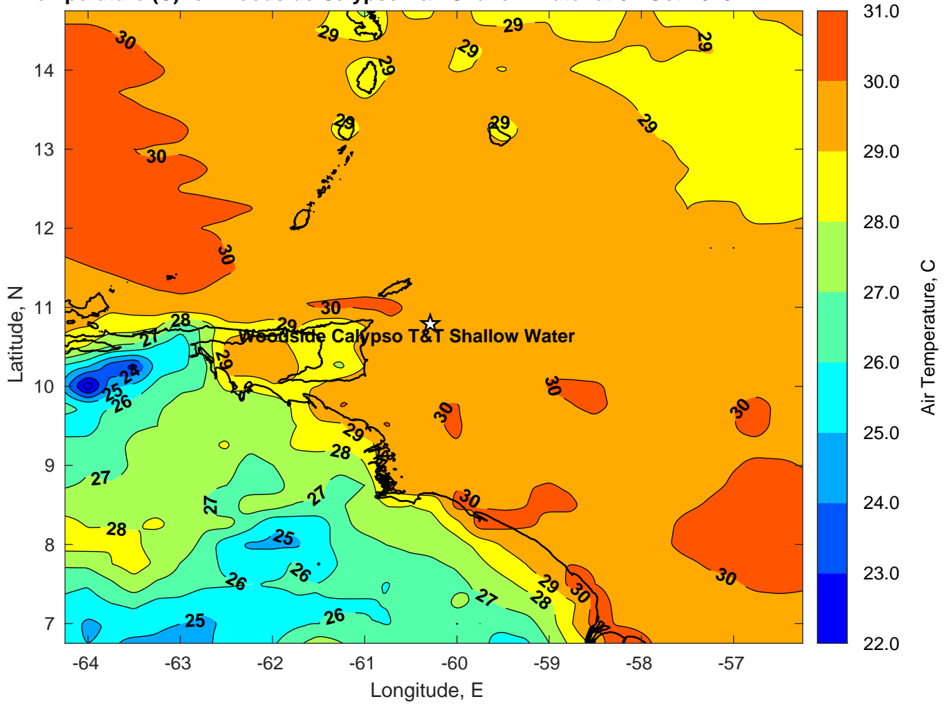
Air Temperature (C) for Woodside Calypso T&T Shallow Water at 31-Oct-2023
