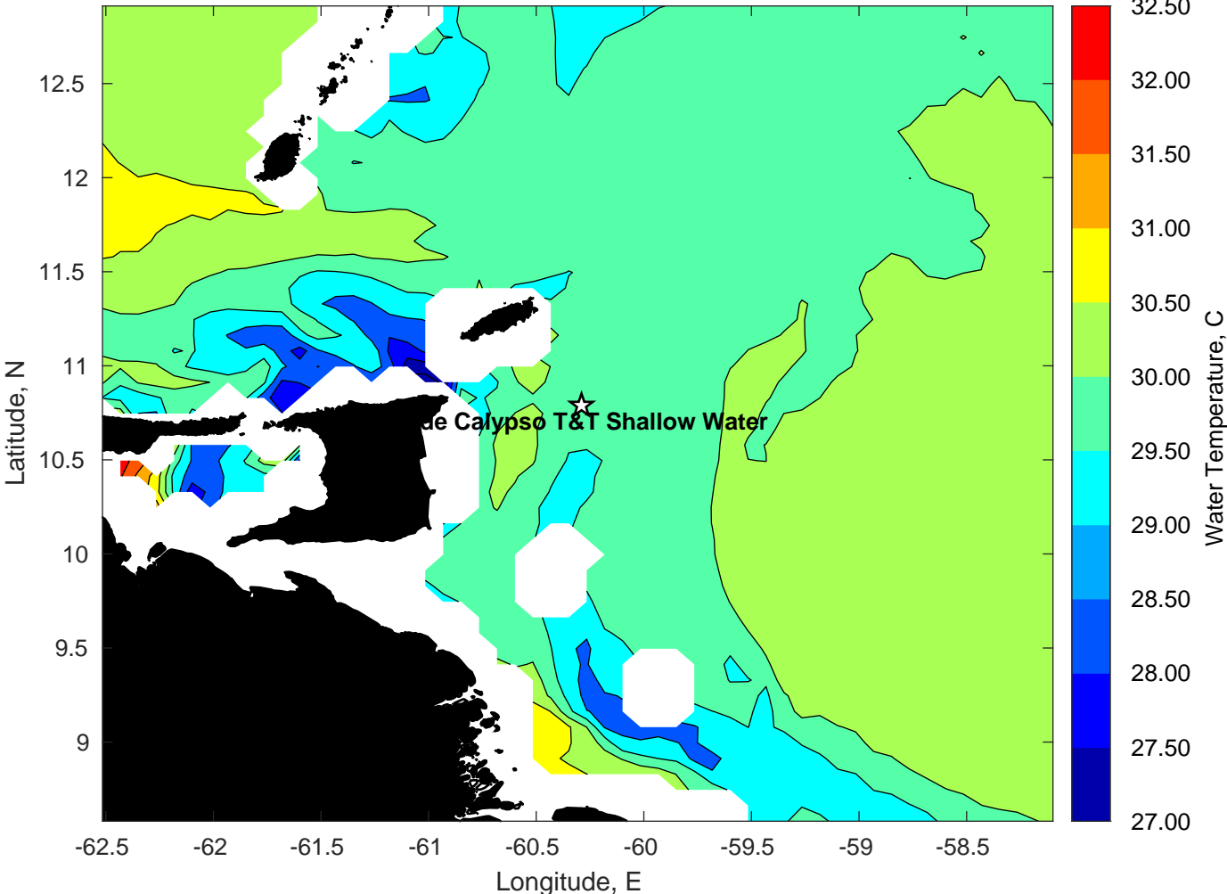
SST for Woodside Calypso T&T Shallow Water at 31-Oct-2023 00:00:00
