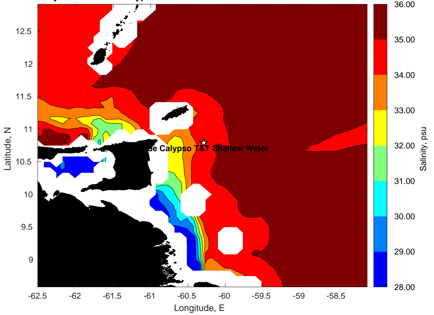
Surface Salinity for Woodside Calypso T&T Shallow Water at 31-Oct-2022 00:00:00
