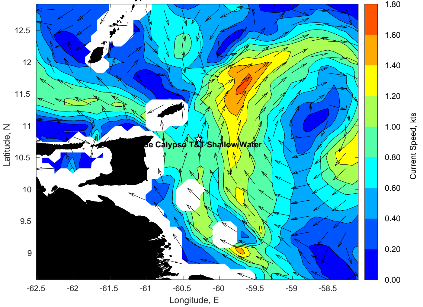
Surface Currents for Woodside Calypso T&T Shallow Water at 31-Oct-2023 00:00:00
