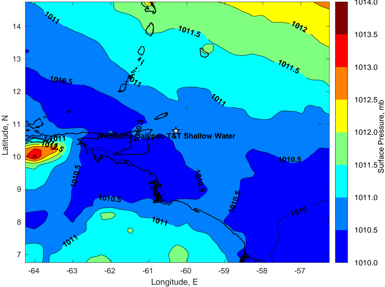
Surface Pressure (mb) for Woodside Calypso T&T Shallow Water at 02-Nov-2023 12:00:00
