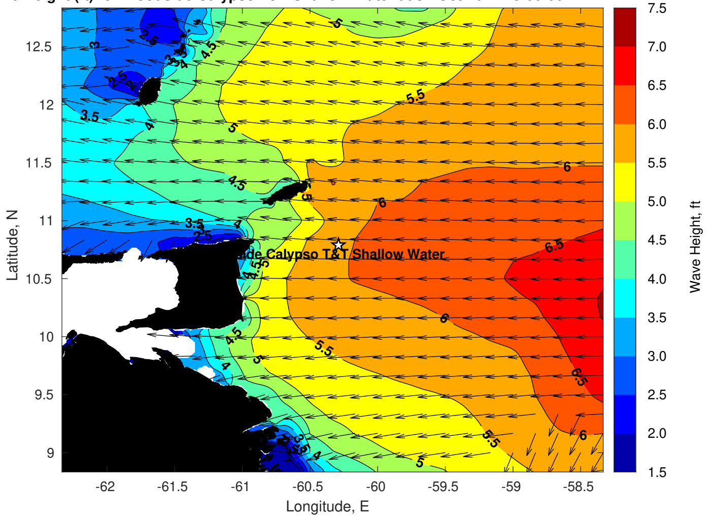
Wave Height (ft) for Woodside Calypso T&T Shallow Water at 31-Oct-2022 18:00:00
