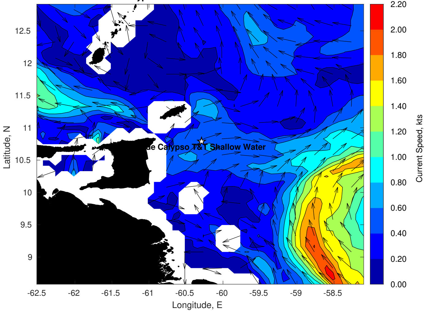
Surface Currents for Woodside Calypso T&T Shallow Water at 31-Oct-2022 00:00:00
