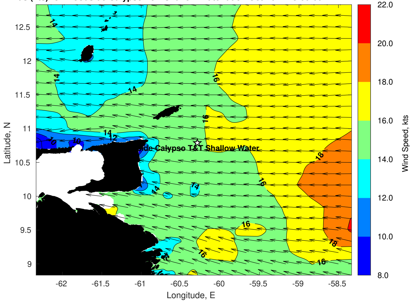
Winds (kts) for Woodside Calypso T&T Shallow Water at 31-Oct-2022 18:00:00
