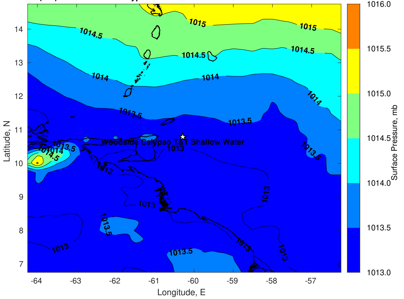
Surface Pressure (mb) for Woodside Calypso T&T Shallow Water at 01-Nov-2022 12:00:00
