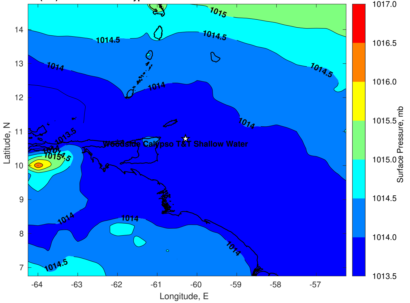
Surface Pressure (mb) for Woodside Calypso T&T Shallow Water at 02-Nov-2022 12:00:00
