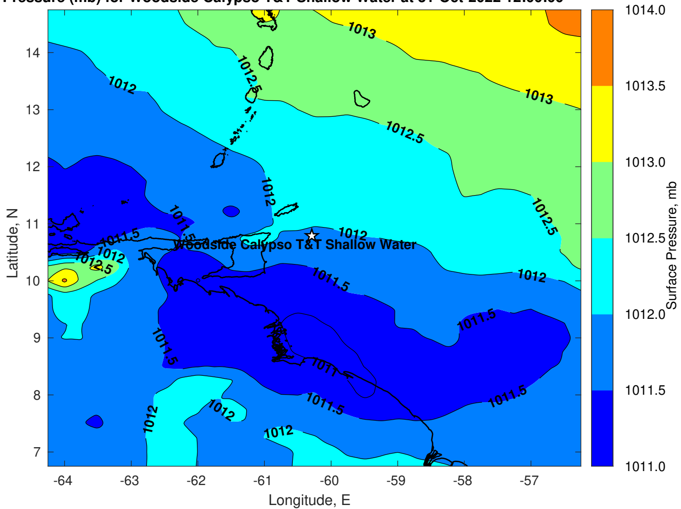
Surface Pressure (mb) for Woodside Calypso T&T Shallow Water at 31-Oct-2022 12:00:00
