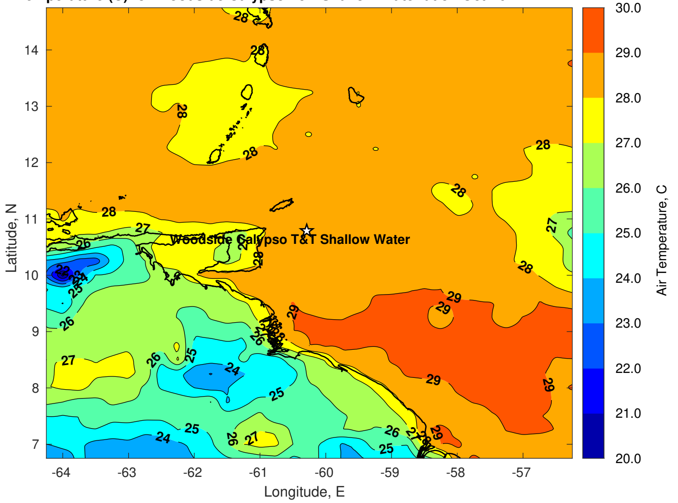
Air Temperature (C) for Woodside Calypso T&T Shallow Water at 31-Oct-2022
