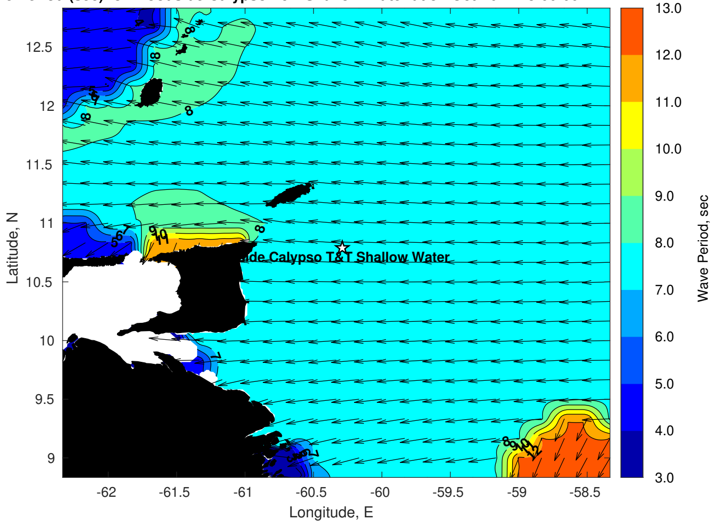
Wave Period (sec) for Woodside Calypso T&T Shallow Water at 31-Oct-2022 18:00:00
