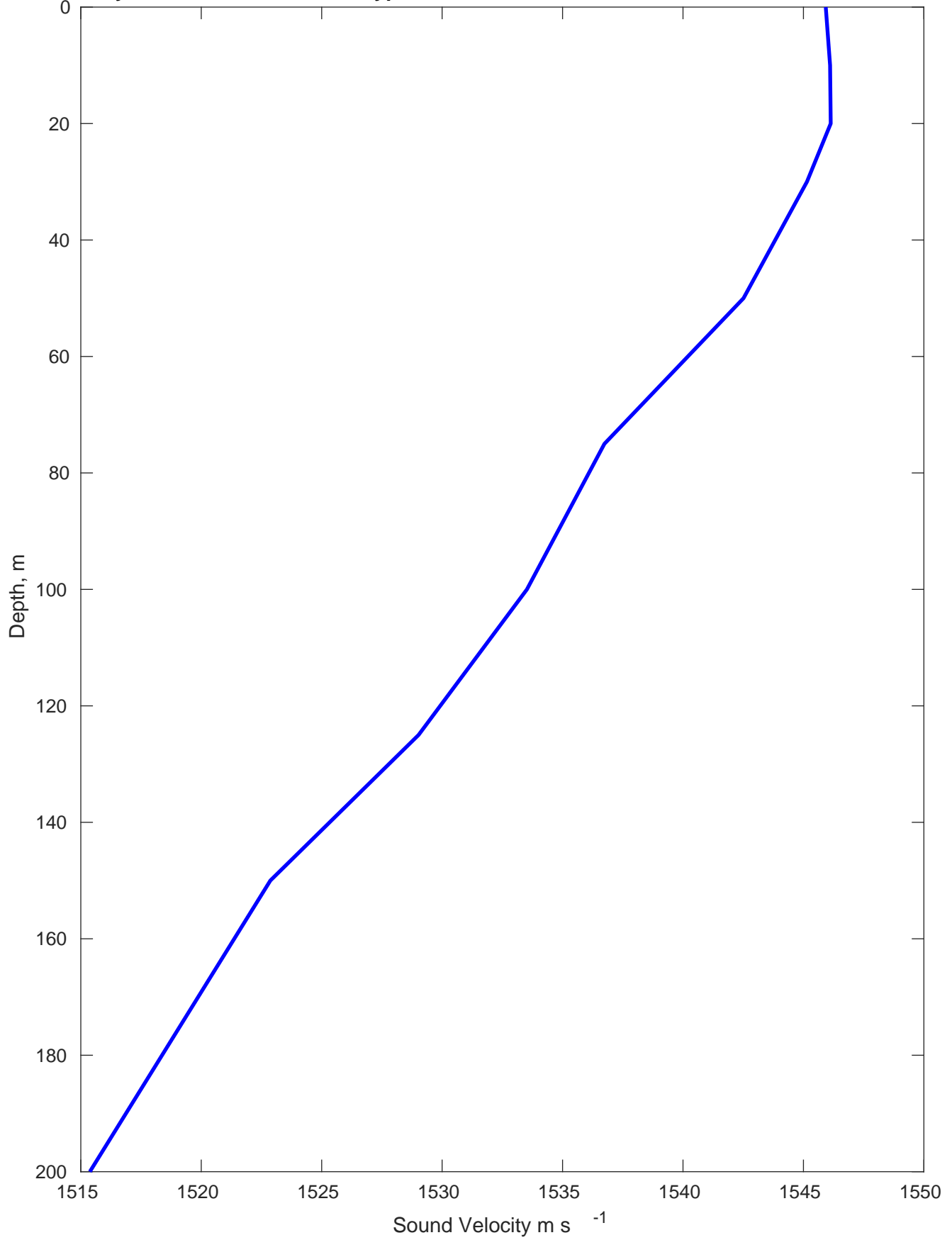
Sound Velocity Profile for Woodside Calypso T&T Shallow Water on 31-Oct-2023 00:00:00
