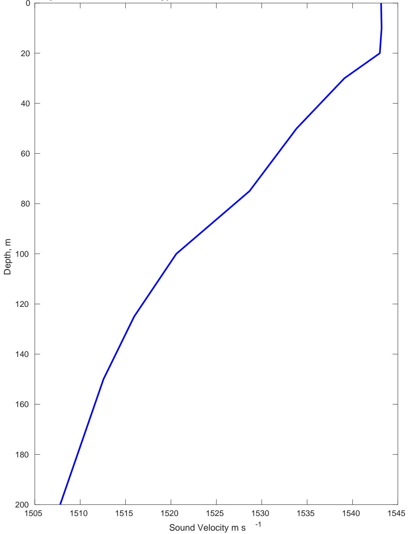
Sound Velocity Profile for Woodside Calypso T&T Shallow Water on 31-Oct-2022 00:00:00
