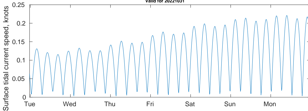
Tidal Currents and Heights for Woodside Calypso T&T Shallow Water at 20221031
