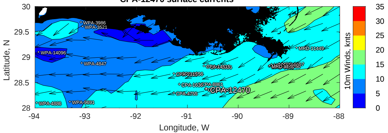
CPA-12470 surface currents
