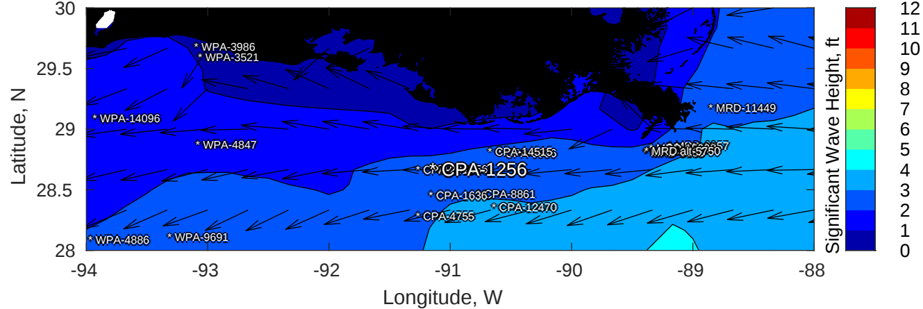
CPA-1256 surface currents
