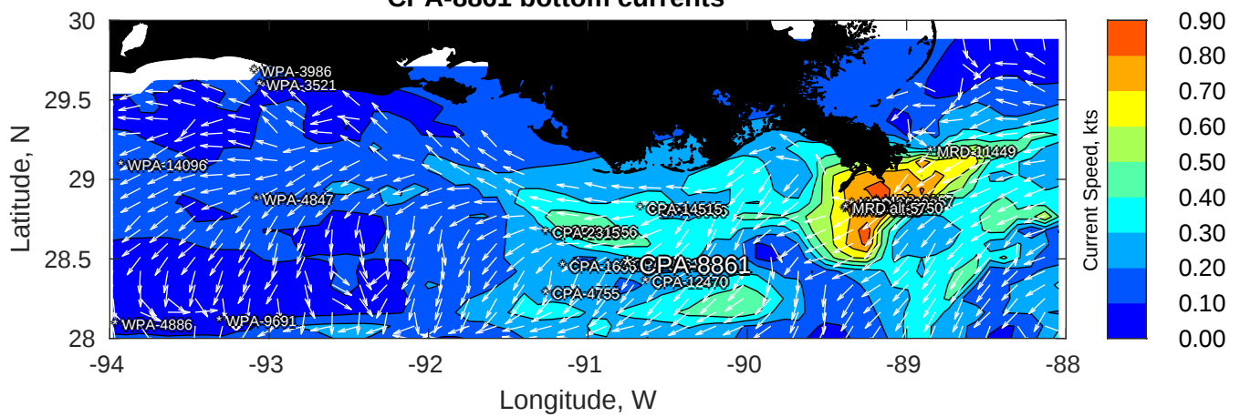
CPA-8861 bottom currents
