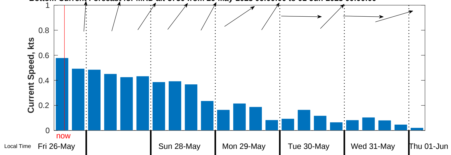
Bottom Current Forecast for MRD alt-5750 from 26-May-2023 06:00:00 to 01-Jun-2023 00:00:00
