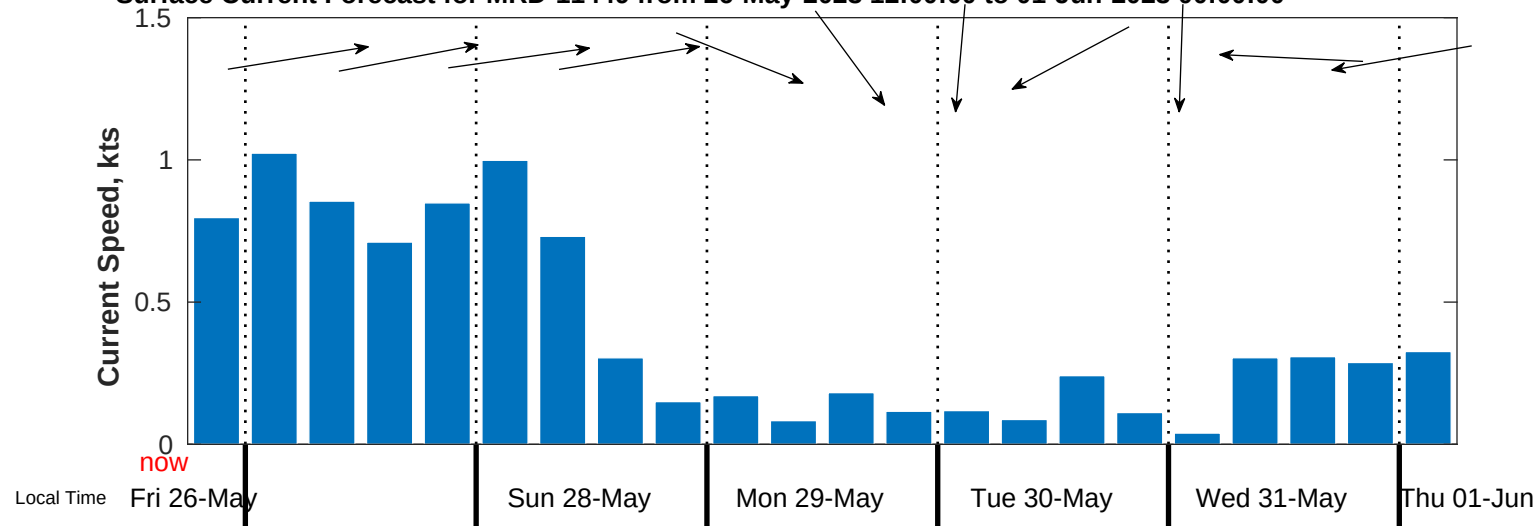
Surface Current Forecast for MRD-11449 from 26-May-2023 12:00:00 to 01-Jun-2023 00:00:00
