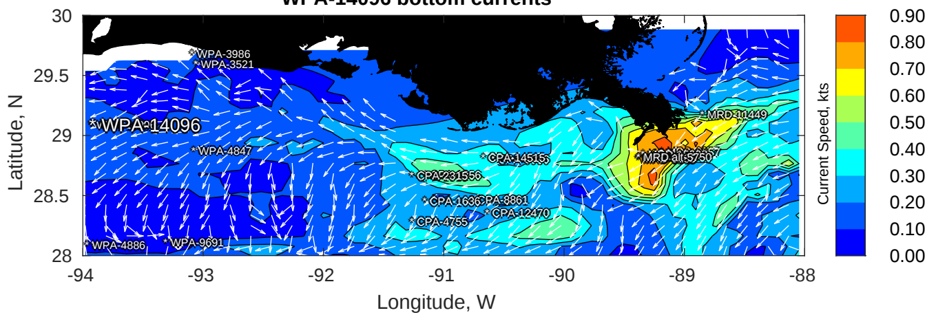
WPA-14096 bottom currents
