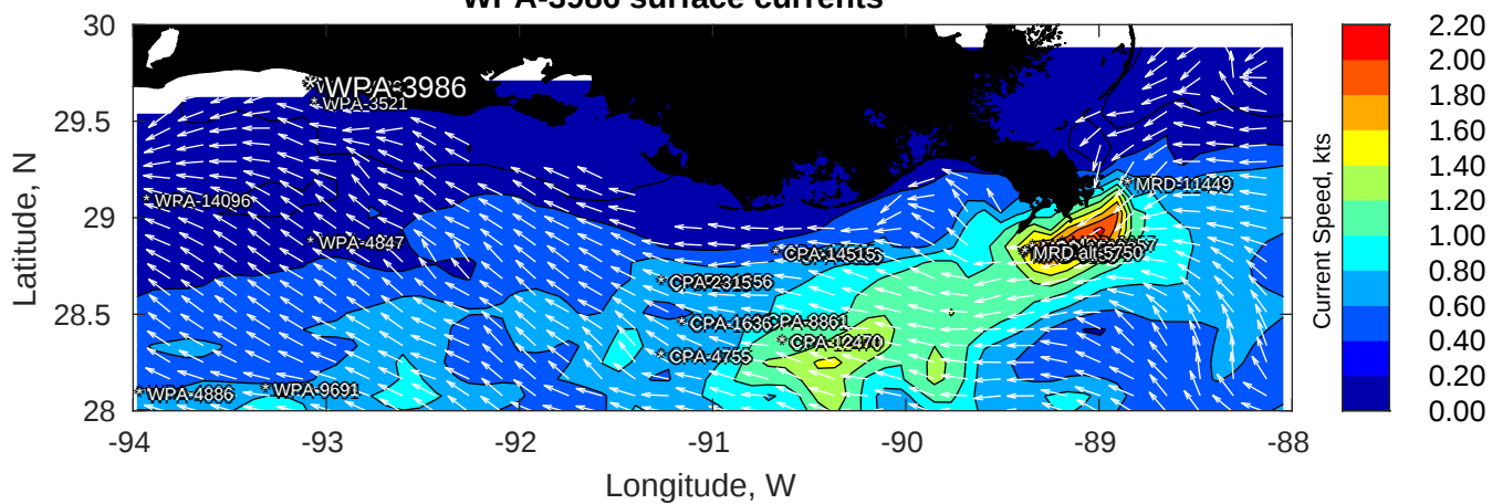
WPA-3986 surface currents
