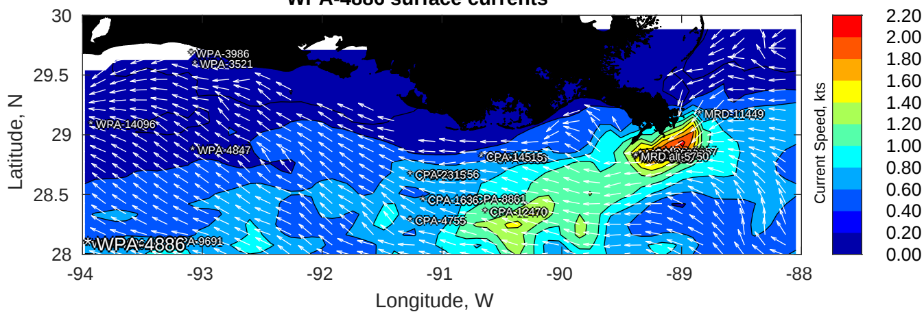
WPA-4886 surface currents
