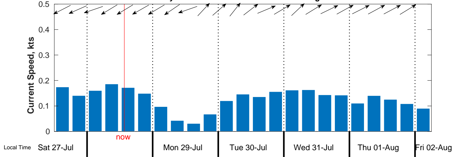
Bottom Current Forecast for Buoy B from 27-Jul-2024 06:00:00 to 02-Aug-2024 00:00:00
