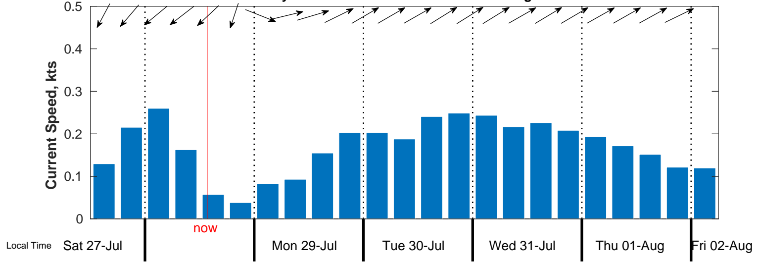
Bottom Current Forecast for Buoy D from 27-Jul-2024 06:00:00 to 02-Aug-2024 00:00:00
