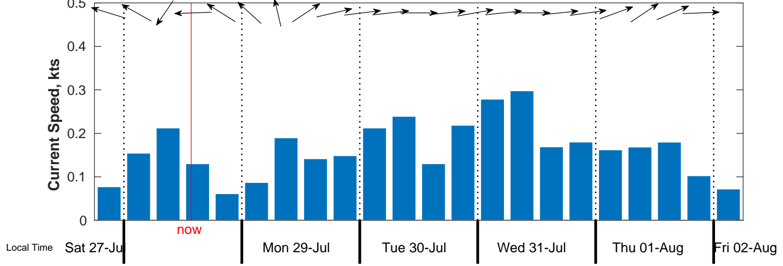
Surface Current Forecast for Buoy F from 27-Jul-2024 12:00:00 to 02-Aug-2024 00:00:00
