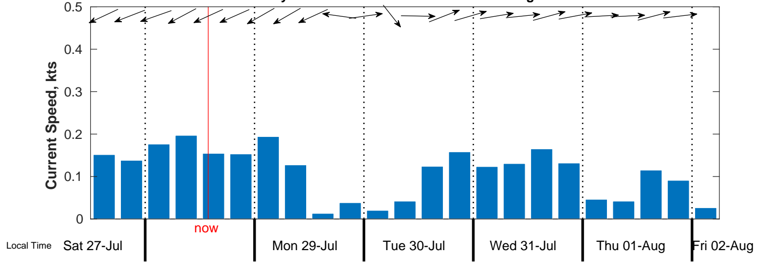
Bottom Current Forecast for Buoy W from 27-Jul-2024 06:00:00 to 02-Aug-2024 00:00:00
