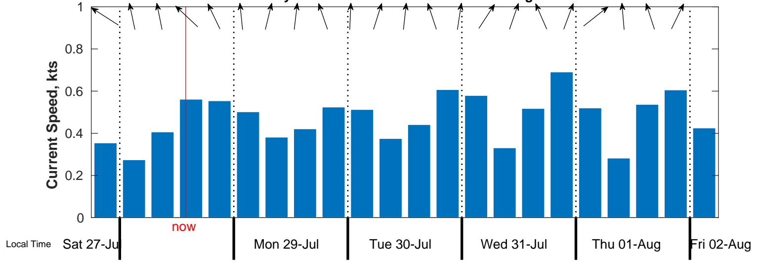
Surface Current Forecast for Buoy X from 27-Jul-2024 12:00:00 to 02-Aug-2024 00:00:00
