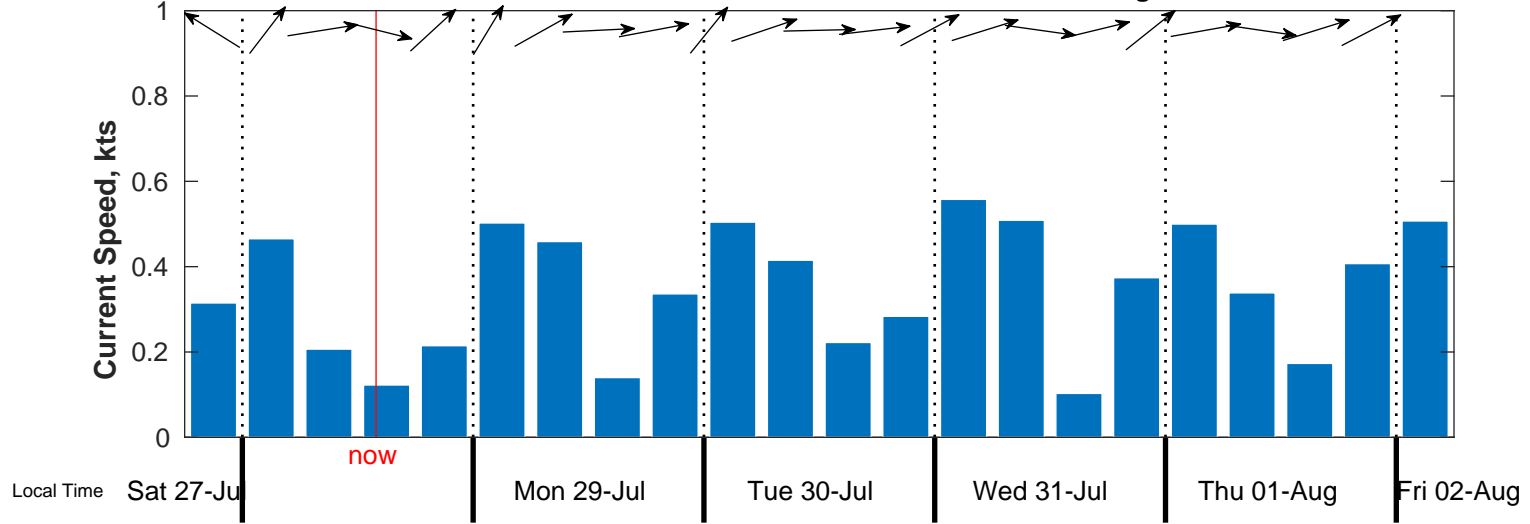
Surface Current Forecast for Flower Gardens NMS from 27-Jul-2024 12:00:00 to 02-Aug-2024 00:00:00
